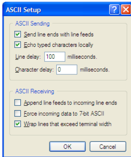
Figure B-5. ASCII Setup Dialog Box
