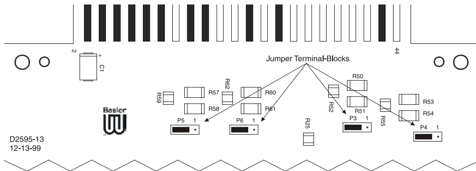
Figure 5-3. Contact Sensing Jumper Locations for 48 Vdc
