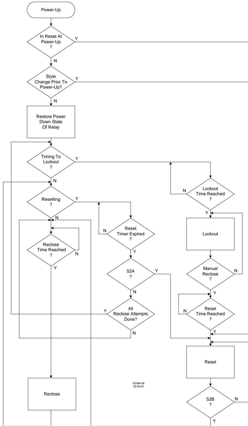
Figure 3-3. Power-Up Flow Chart
