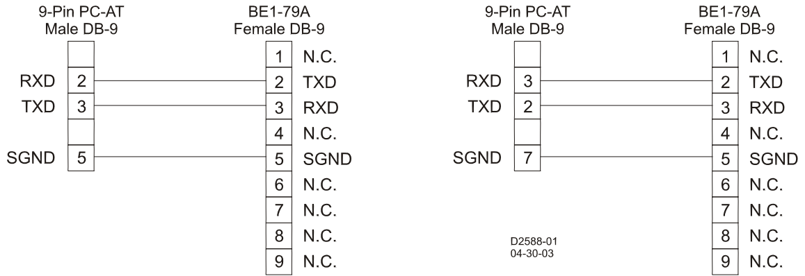
Figure 5-6. PC to BE1-79A Connections
