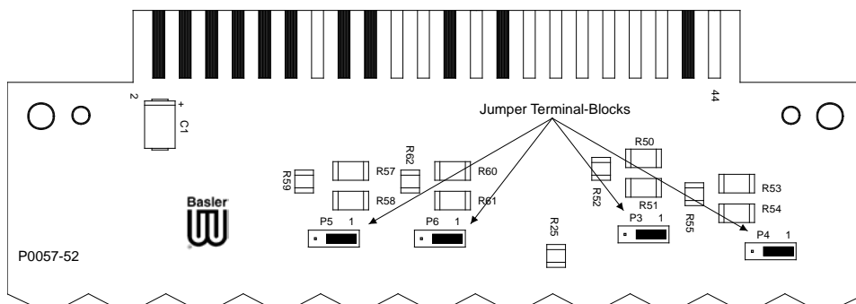
Figure 5-4. Contact Sensing Jumper Locations for 125 Vdc or 120 Vac
