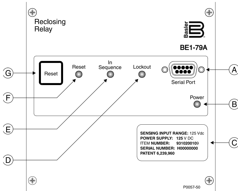
Figure 2-1. Front Panel Controls and Indicators
