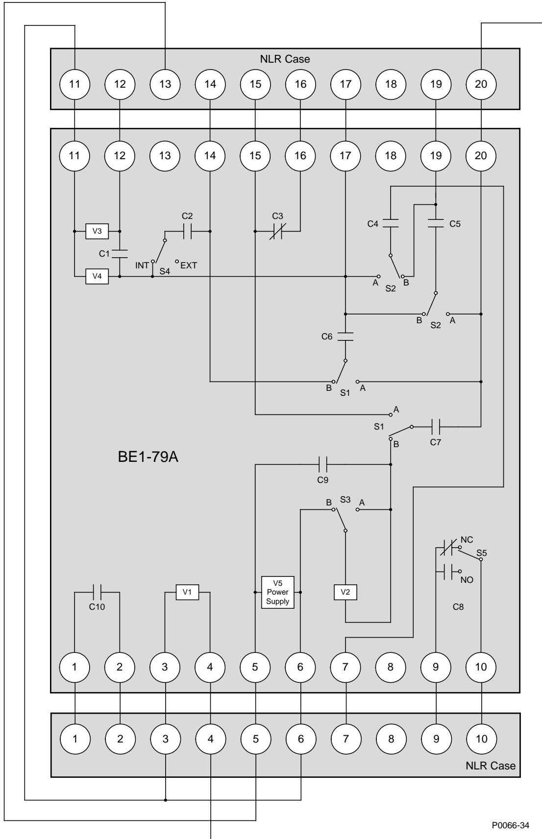
Figure 5-1. Relay Connections
