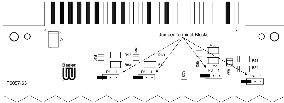
Figure 5-5. Contact Sensing Jumper Locations for 250 Vdc or 240 Vac
