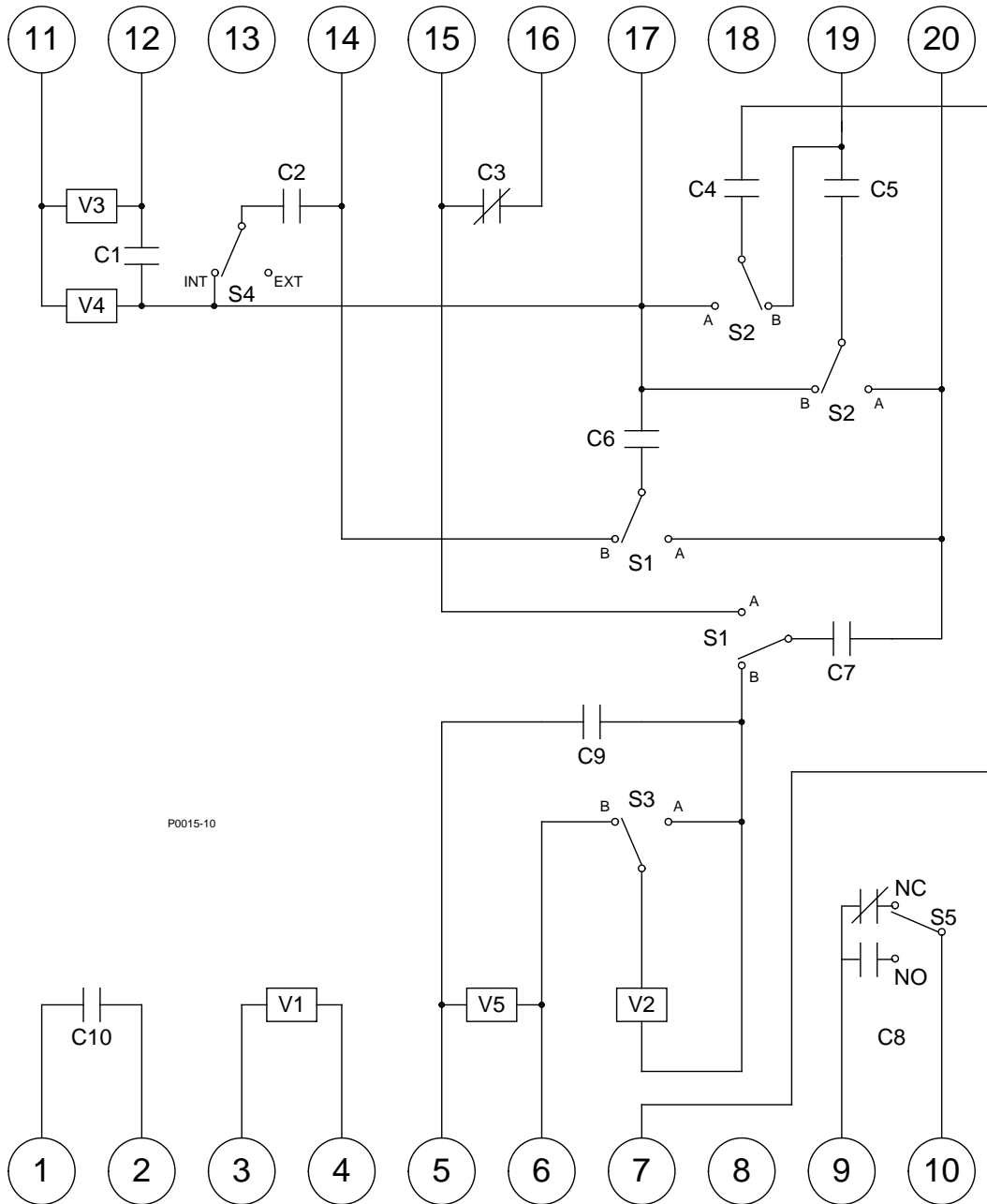
Figure 3-2. Relay Interconnections for NLR-21U Applications
