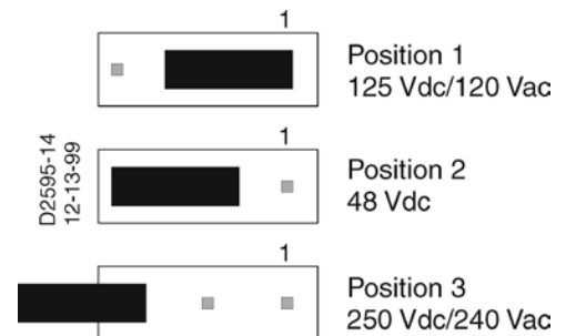
Figure 5-2. Contact Sensing Jumpers
