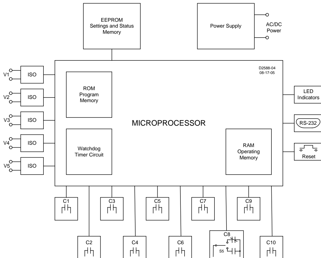
Figure 3-1. Function Block Diagram
