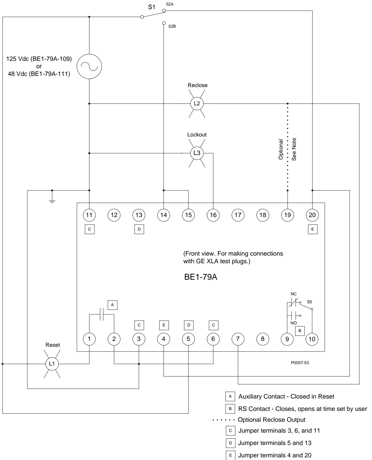
Figure 6-1. Test Connections for NLR-21U Relays
