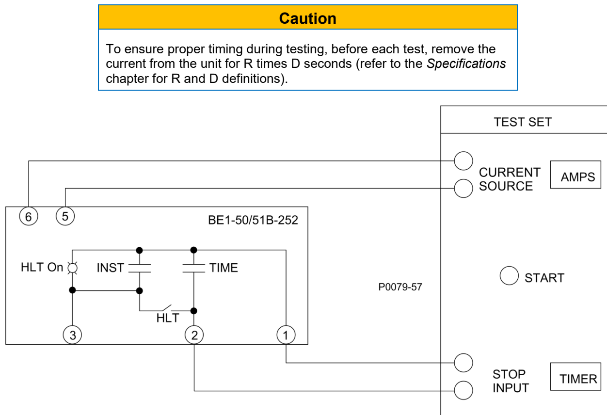
Figure 5-1. Pickup and Timing Test Setup
