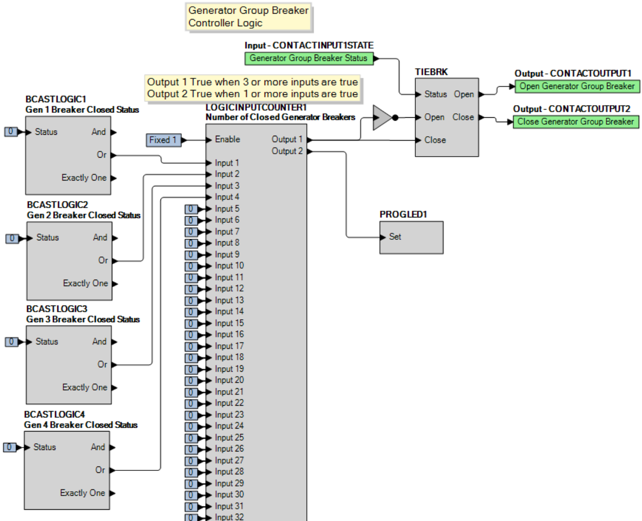
Figure 15. Generator Goup Breaker Controller Logic
