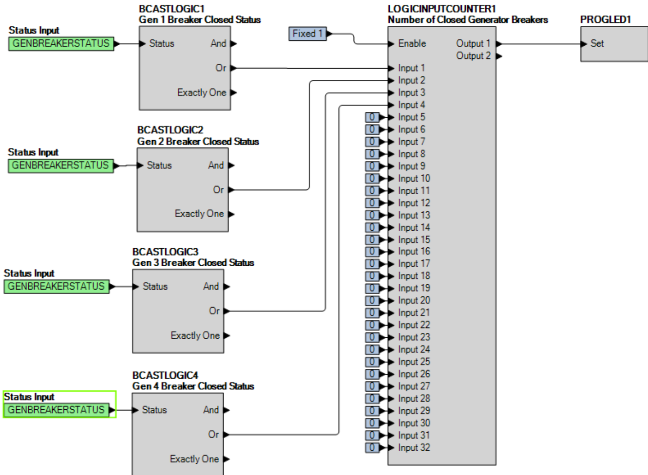
Figure 16. Live Generator Bus Indication Logic
