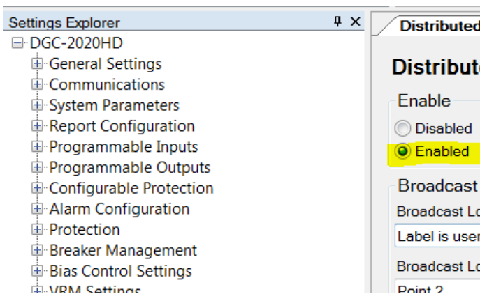
Figure 1. Distributed Logic Broadcast Tab
