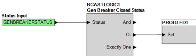
Figure 11. Generator Breaker Annunciation Logic
