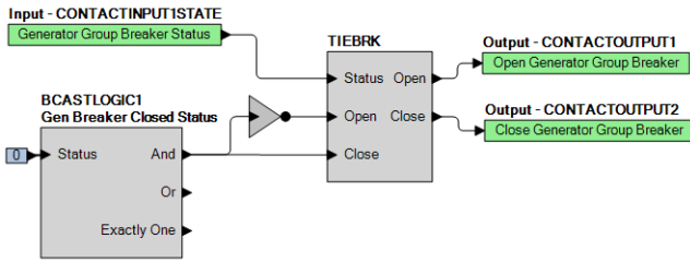
Figure 10. Generator Group Breaker Logic
