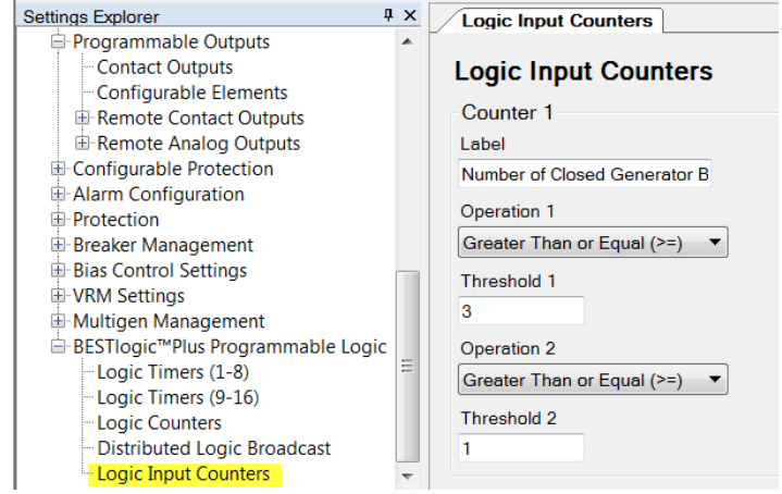
Figure 14. Logic Input Counter Settings
