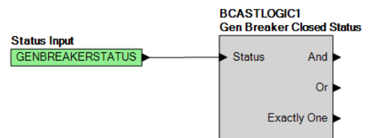
Figure 9. Broadcast Logic 1 Element Driven by the Generator Breaker Status
