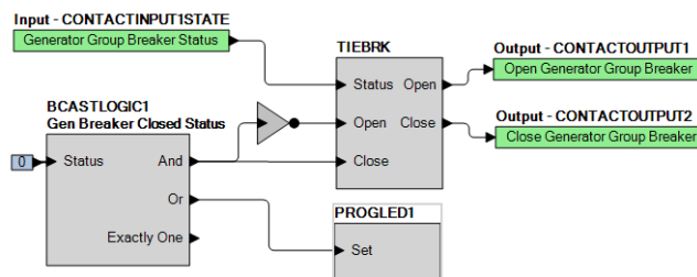
Figure 12. Generator Group Breaker Annunciation Logic
