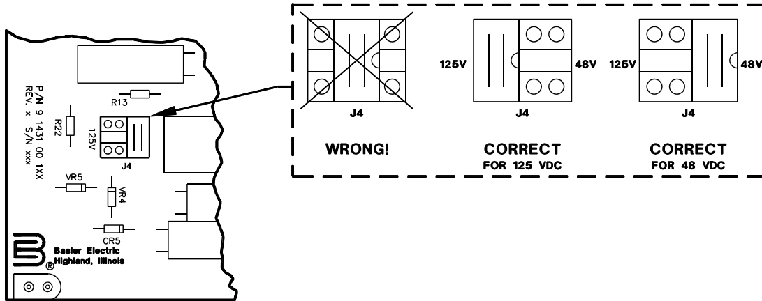
Figure 3-2. J4 Link Positioning
