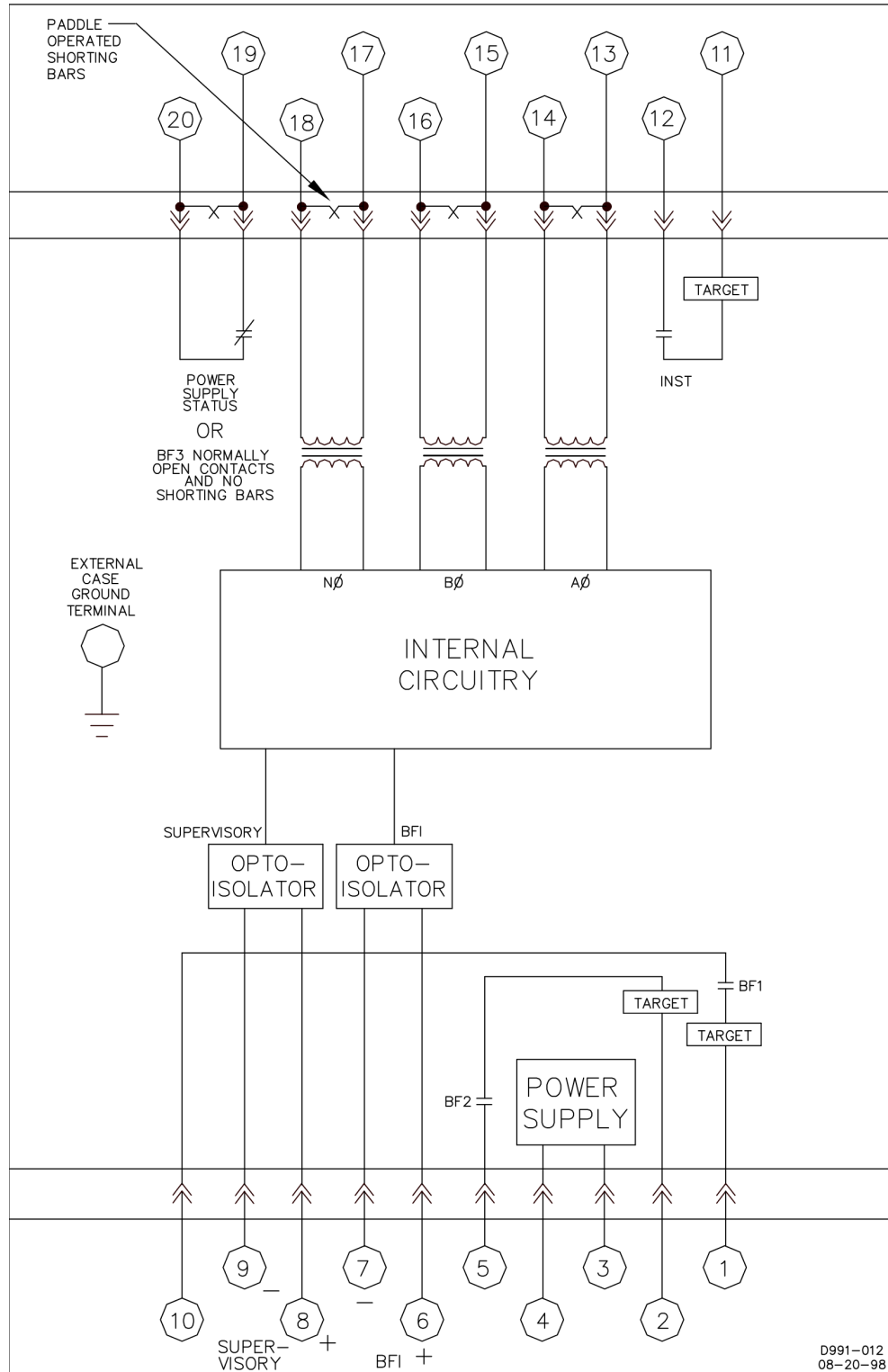
Figure 4-8. Typical Internal Connections, Sensing Input Type E
