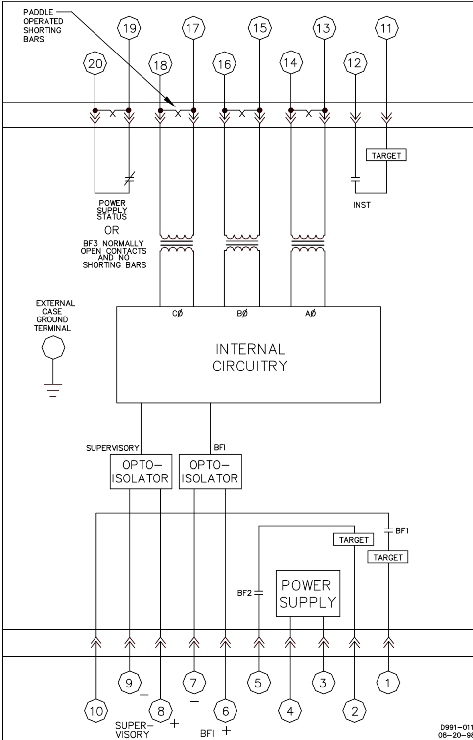
Figure 4-9. Typical Internal Connections, Sensing Input Type F
