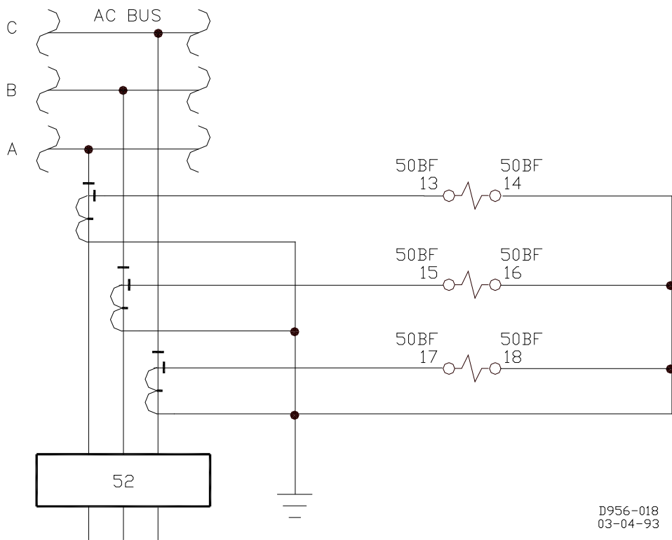
Figure 4-13. Typical Connections Sensing Input Type F
