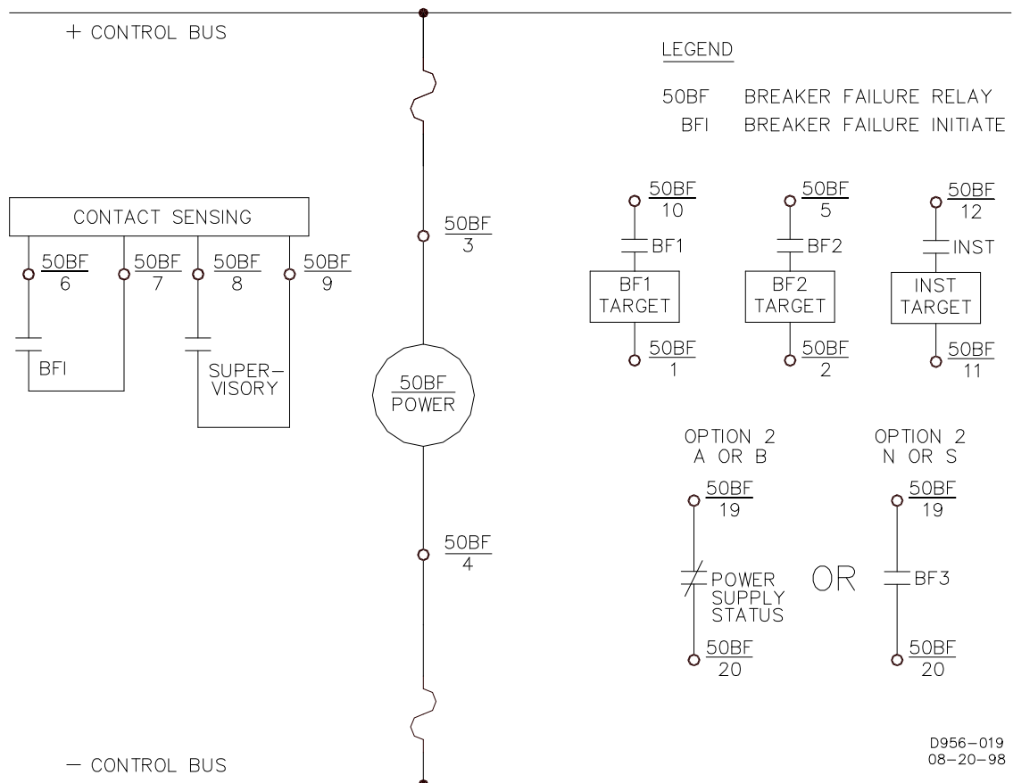
Figure 4-11. Control Circuit Connections (Typical) Isolated Inputs
