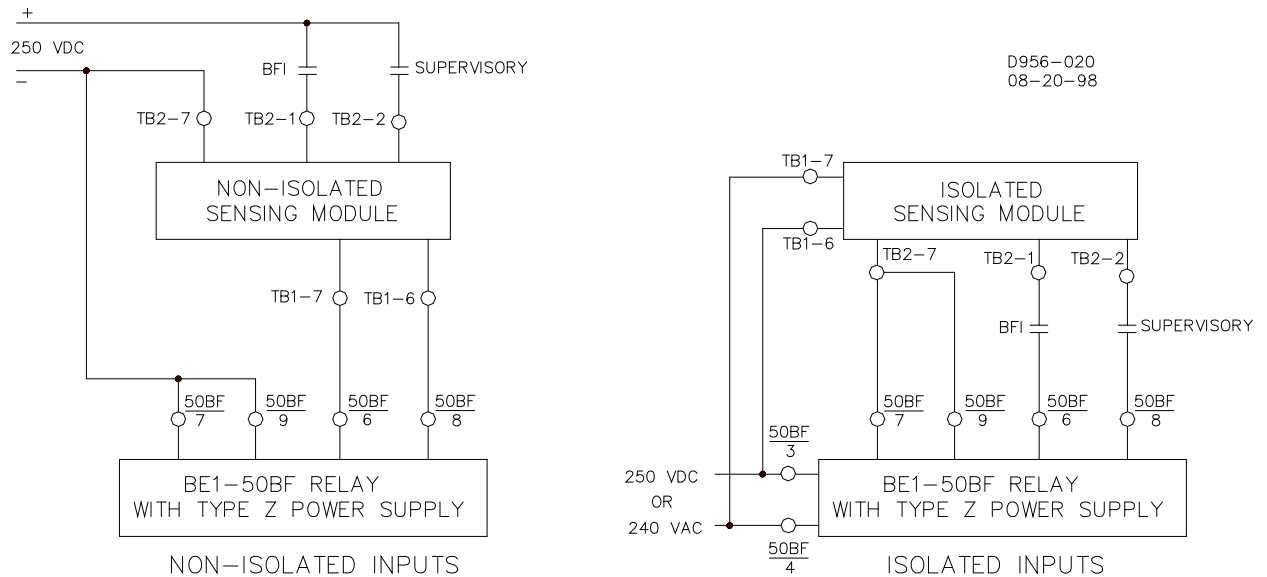
Figure 4-14. Contact Sensing Modules, Power Supply Z
