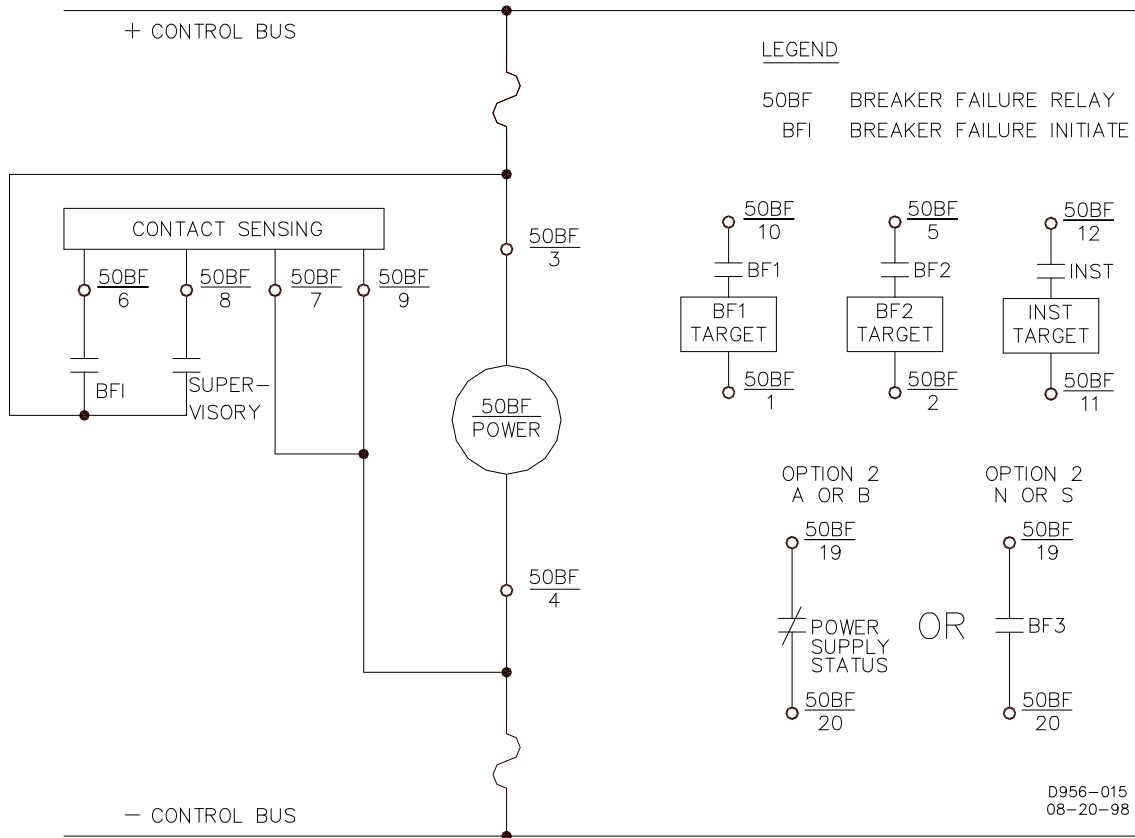
Figure 4-10. Control Circuit Connections (Typical) Non-Isolated Inputs
