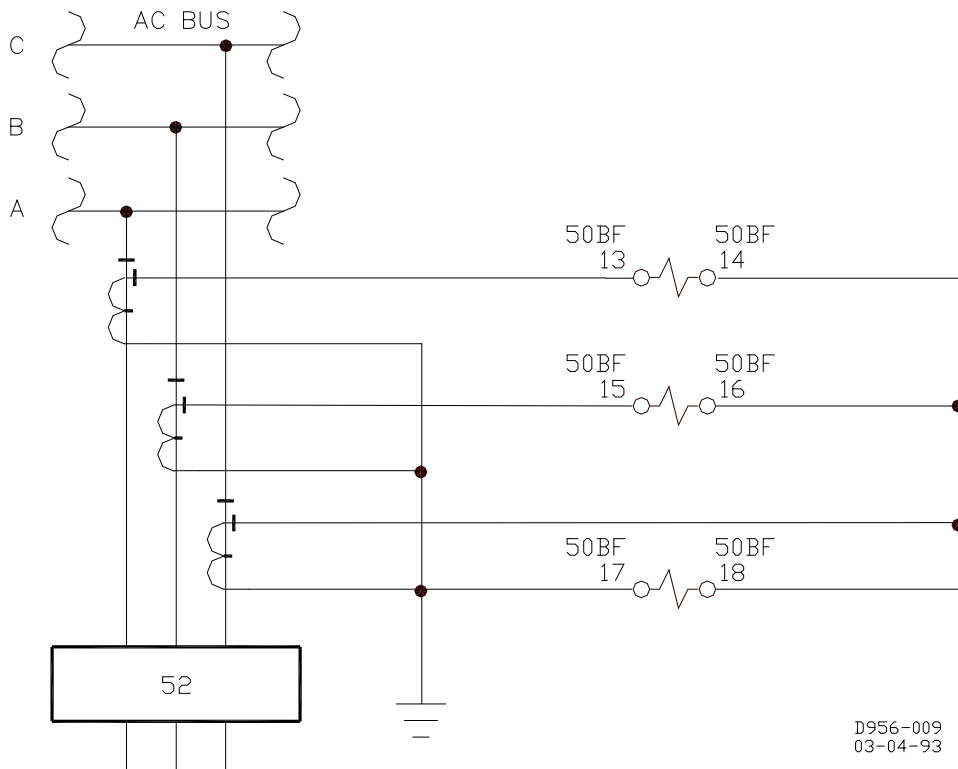
Figure 4-12. Typical Connections Sensing Input Type E
