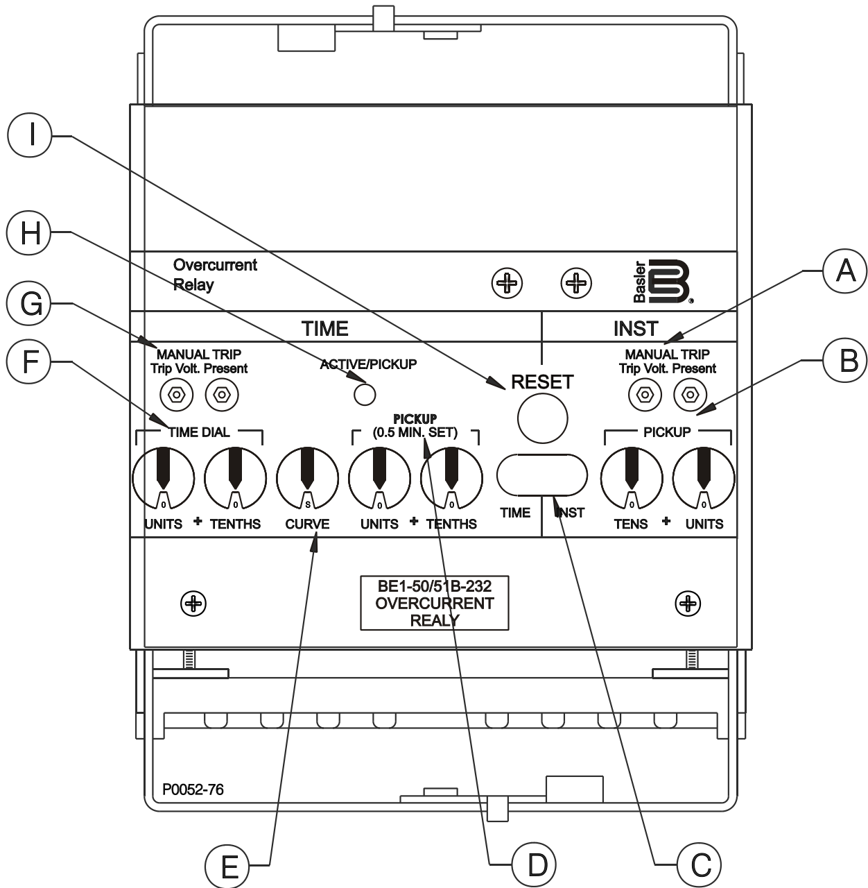
Figure 2-1. Front Panel Controls and Indicators
