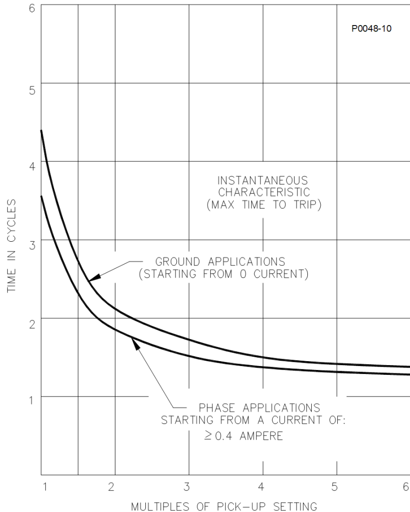
Figure 6-2. Instantaneous Characteristic Curves
