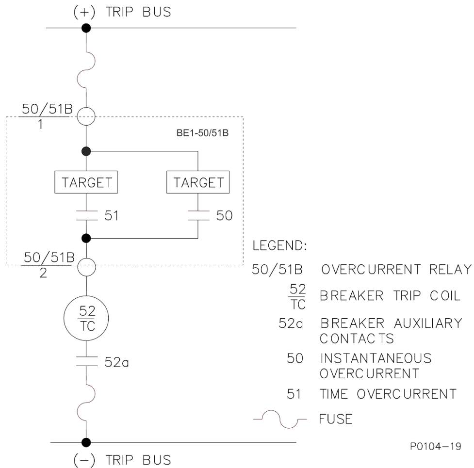
Figure 4-7. DC Control Connections
