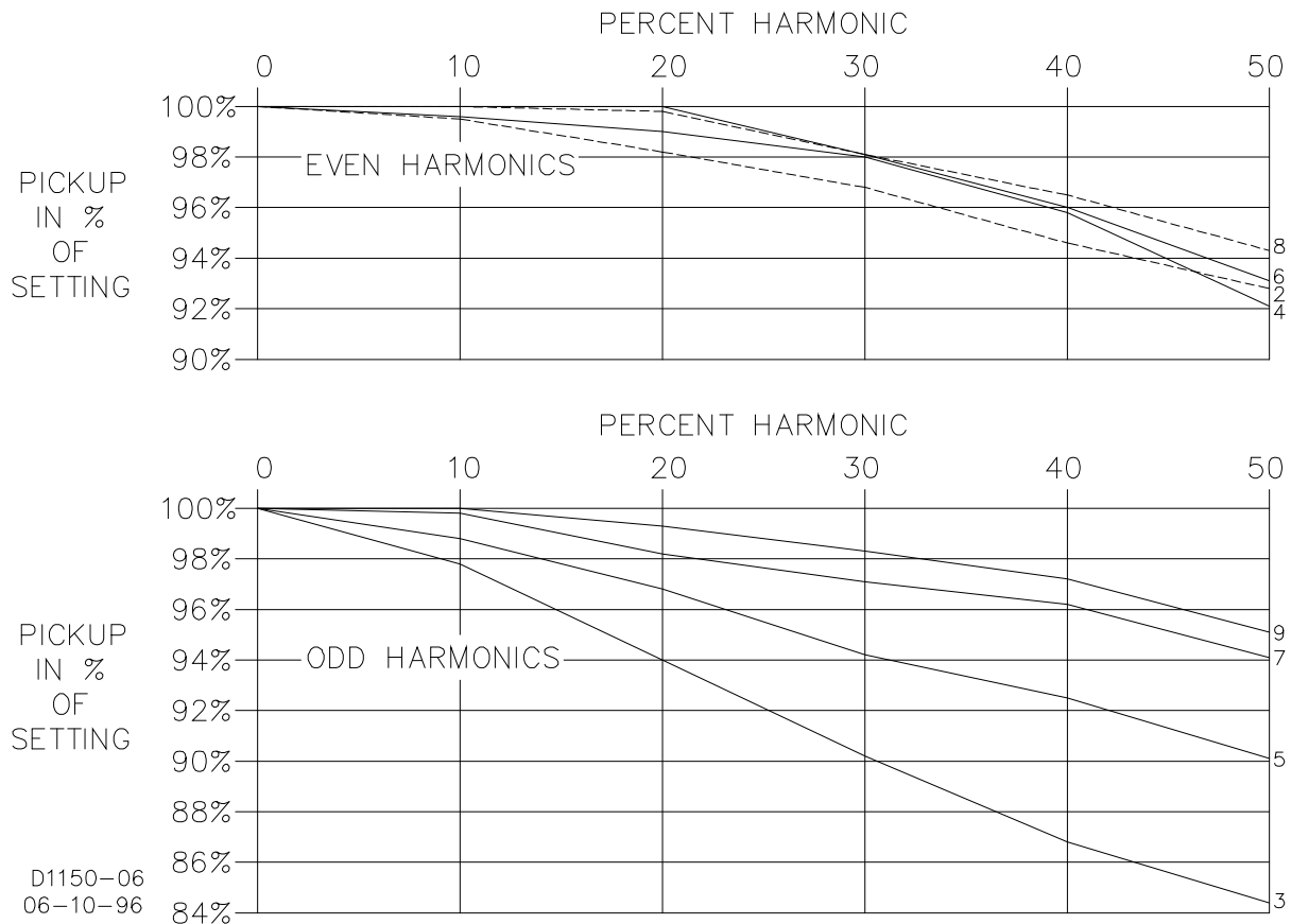
Figure 6-4. Harmonic Rejection
