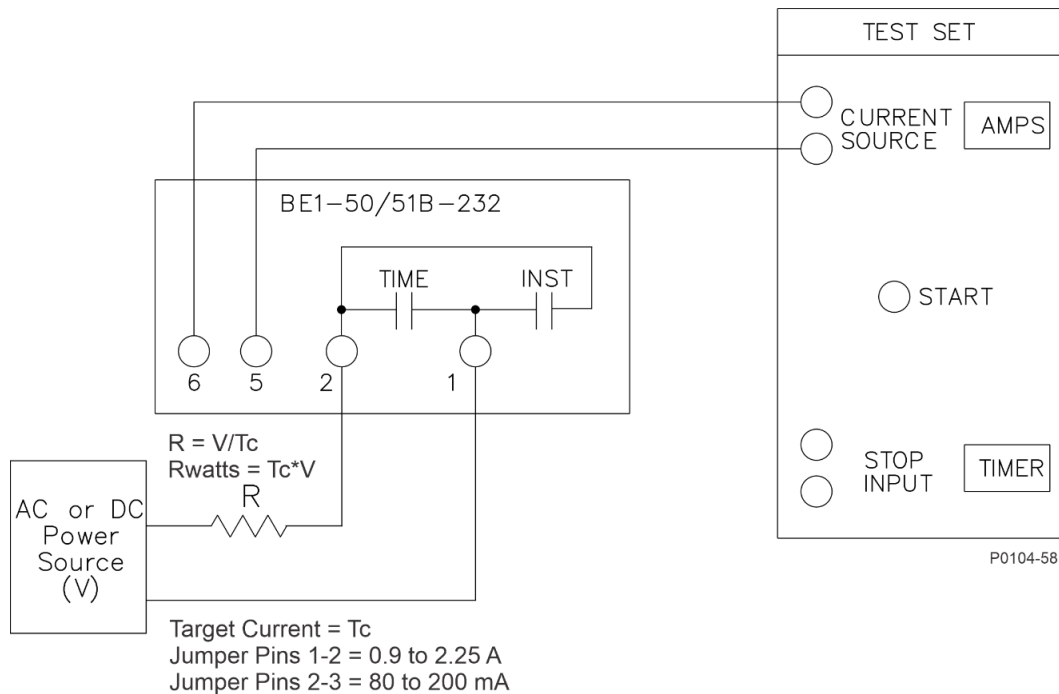
Figure 5-2. Target Operational Test Setup
