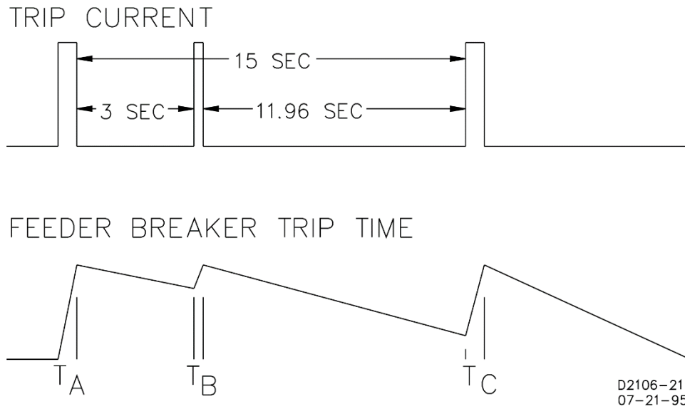
Figure 4-5. Coordination Timing Diagram
