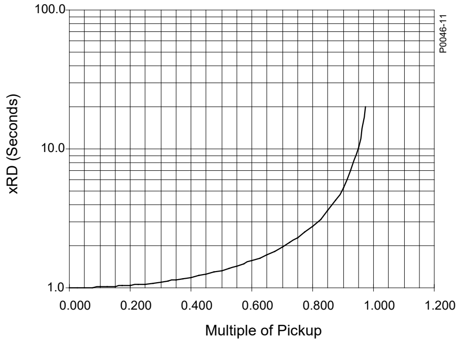
Figure 6-1. Integrating Reset Characteristic Curve
