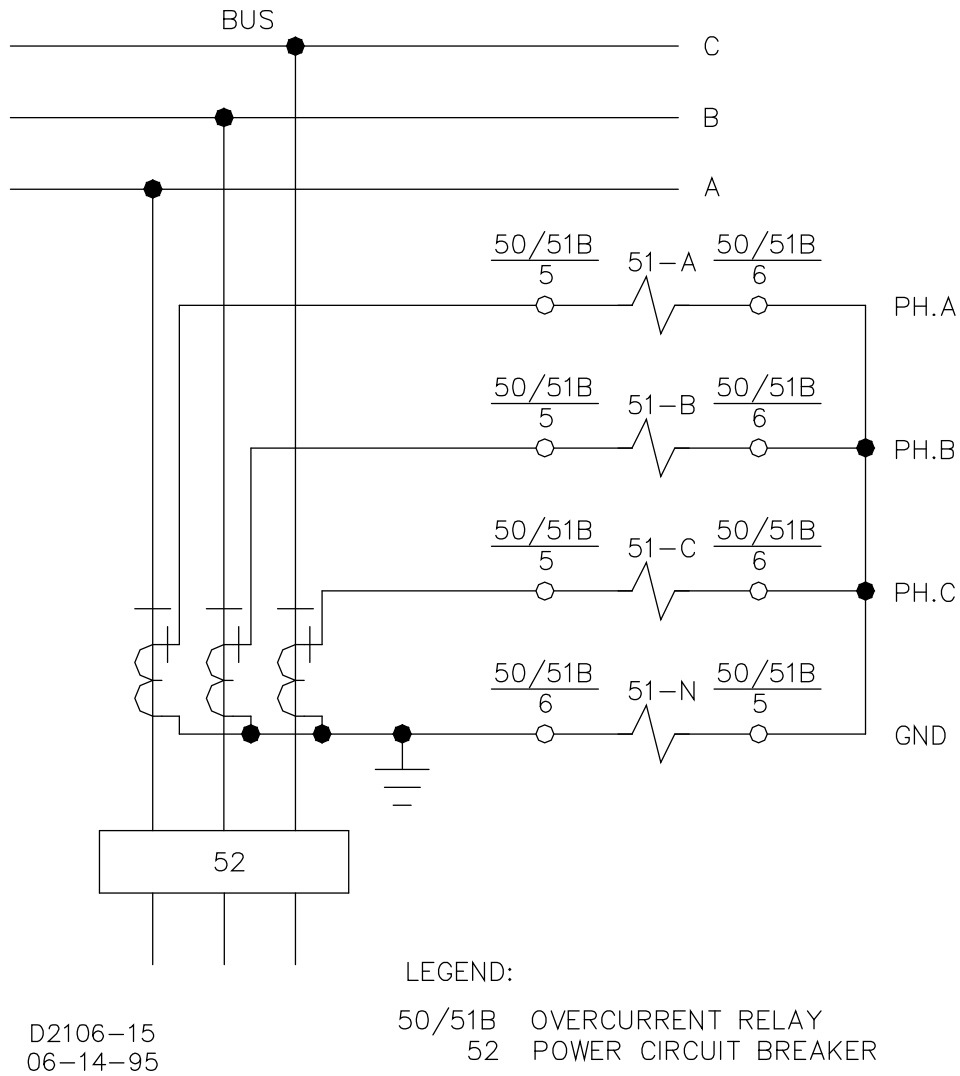
Figure 4-6. AC Input Connections
