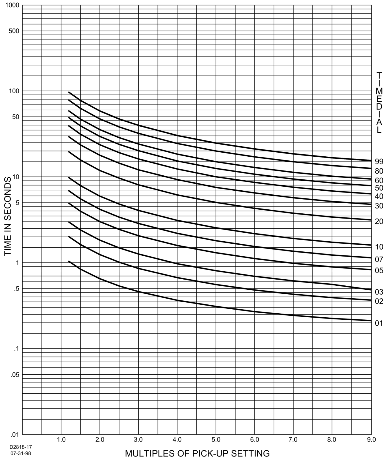
Figure 3-2. Negative Sequence Voltage Inverse Time Characteristic Curves
