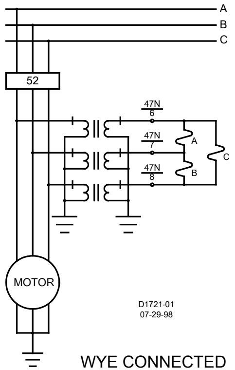
Figure 4-9. Sensing Input Connection
