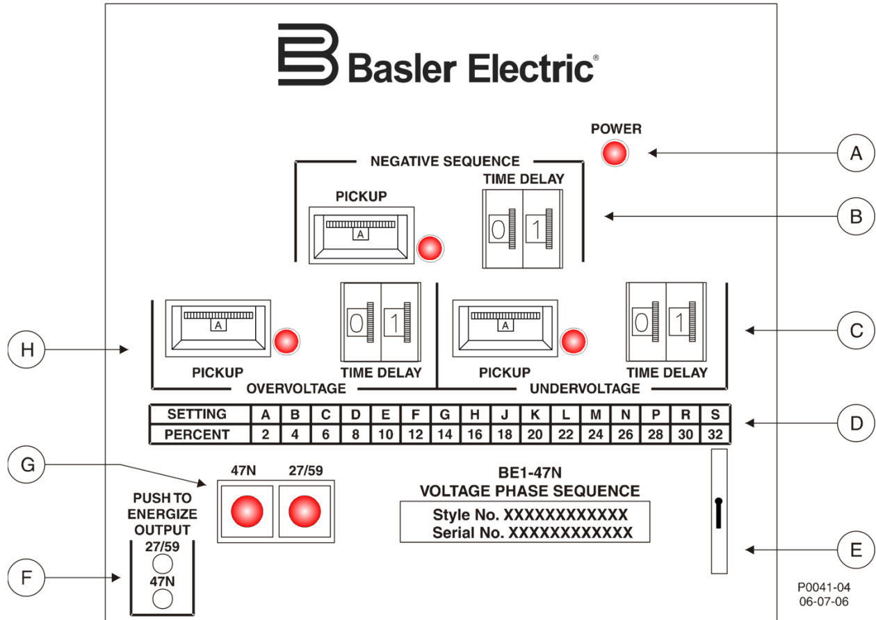
Figure 2-1. BE1-47N Controls and Indicators
