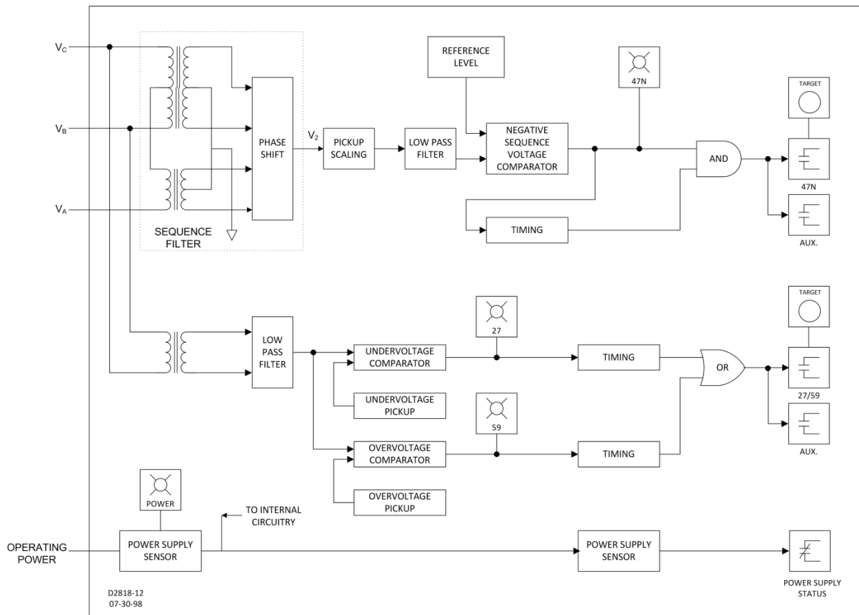
Figure 3-1. Function Block Diagram
