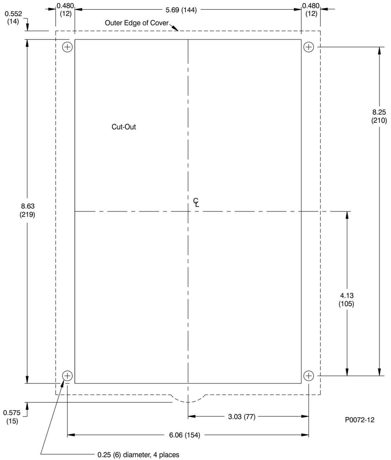
Figure 4-1. Panel Cutting/Drilling, Semi-Flush, S1 Case
