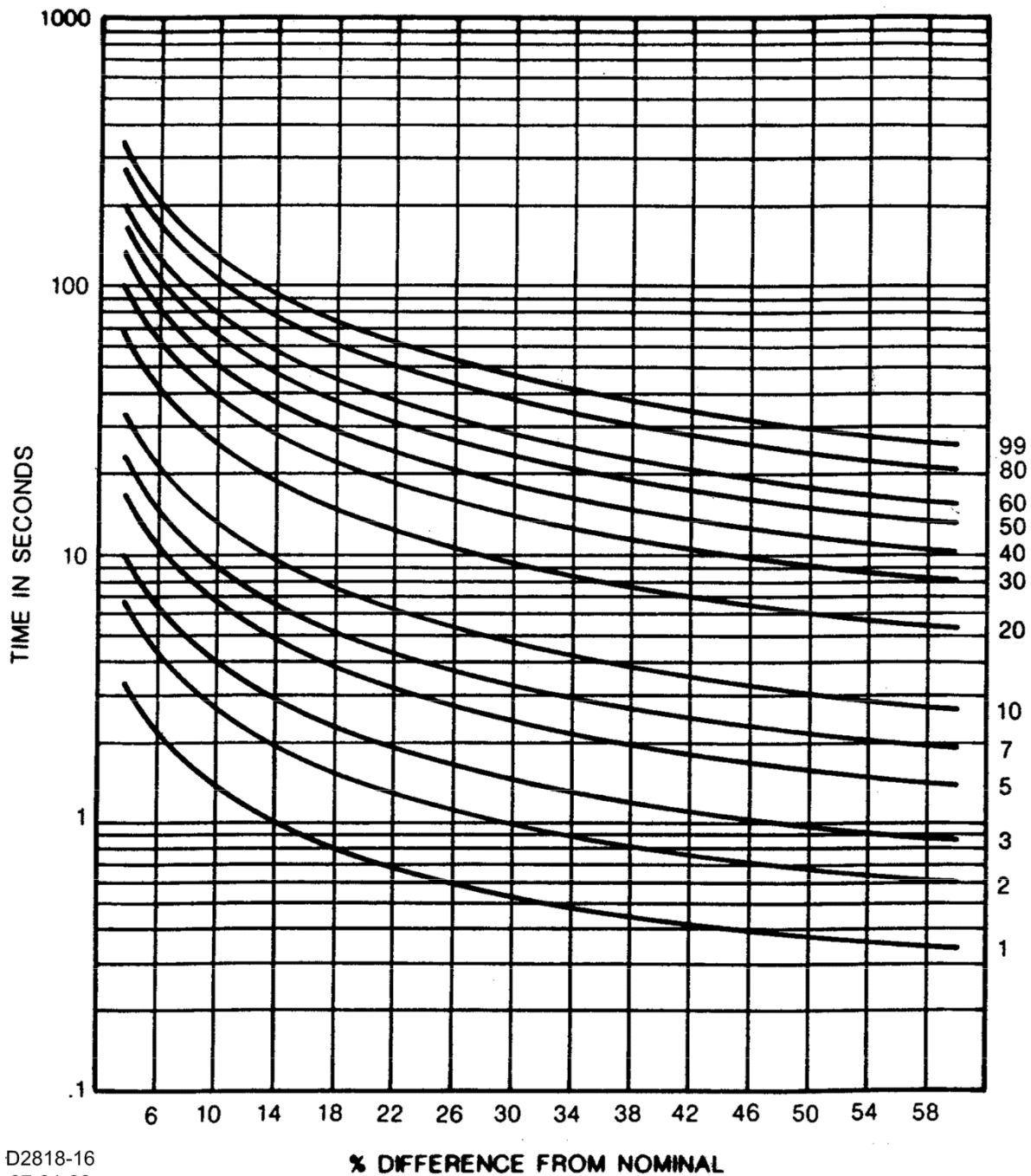
Figure 3-4. Overvoltage Inverse Time Characteristic Curves
