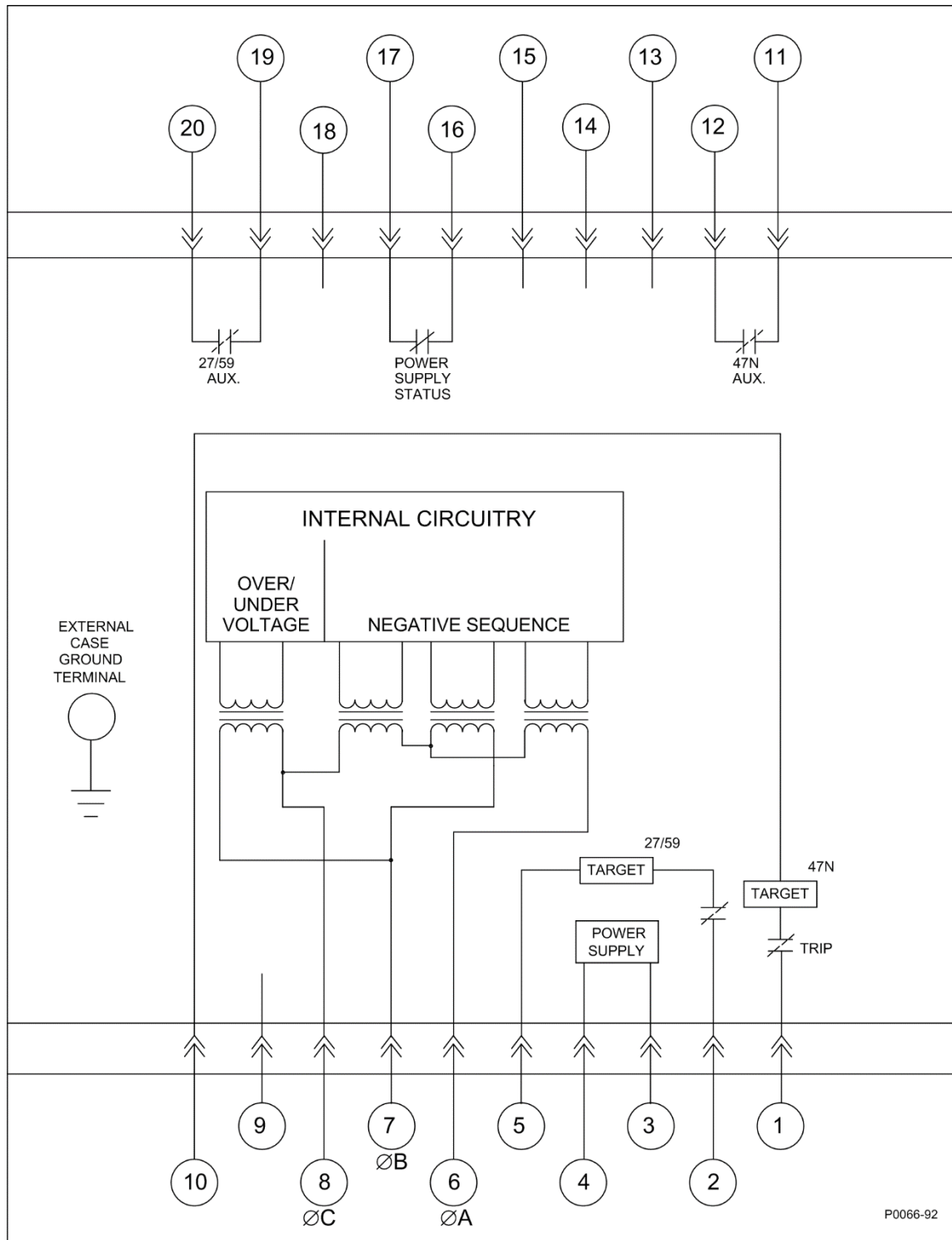
Figure 4-10. Typical Internal Connection Diagram
