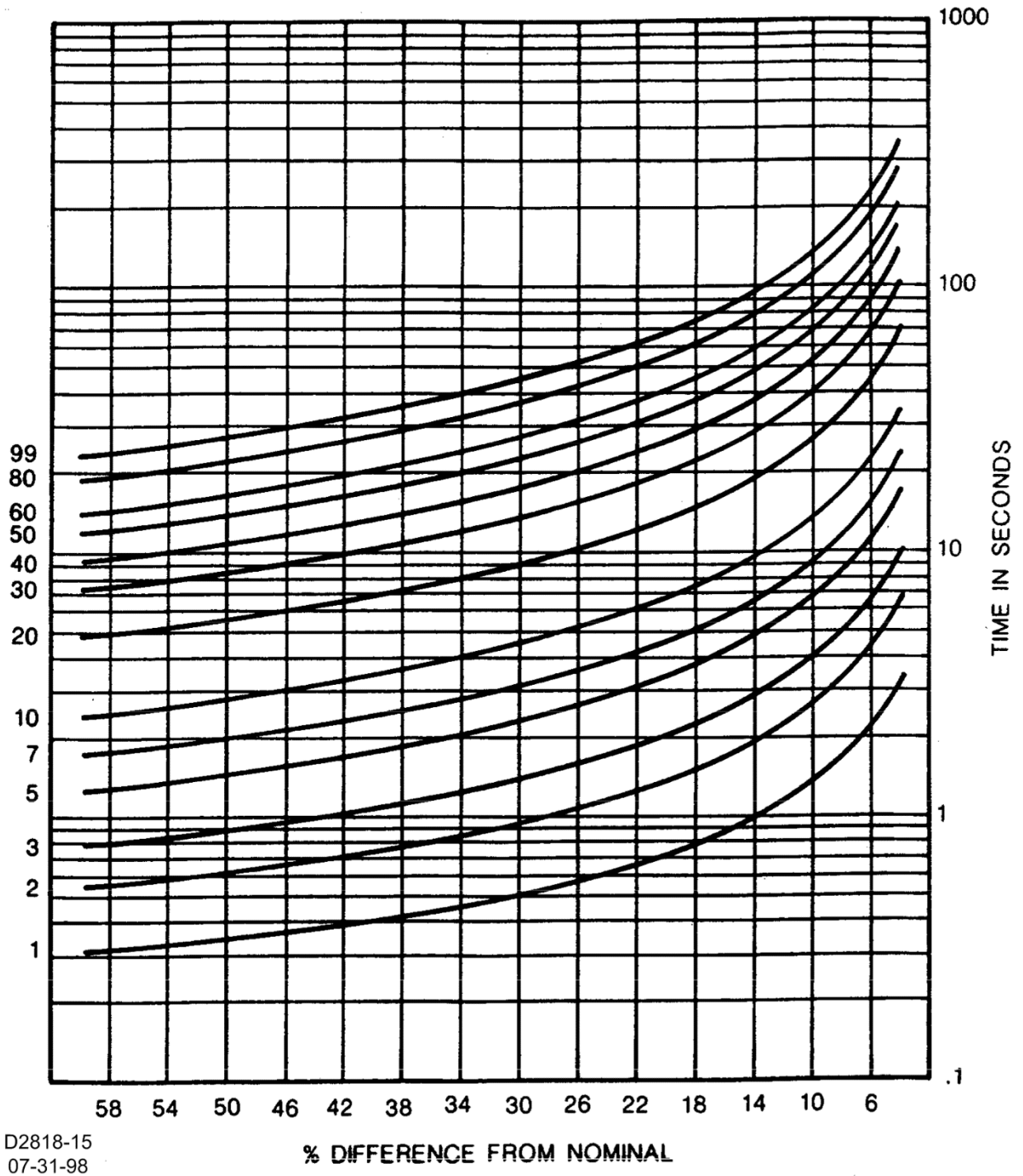
Figure 3-3. Undervoltage Inverse Time Characteristic Curves
