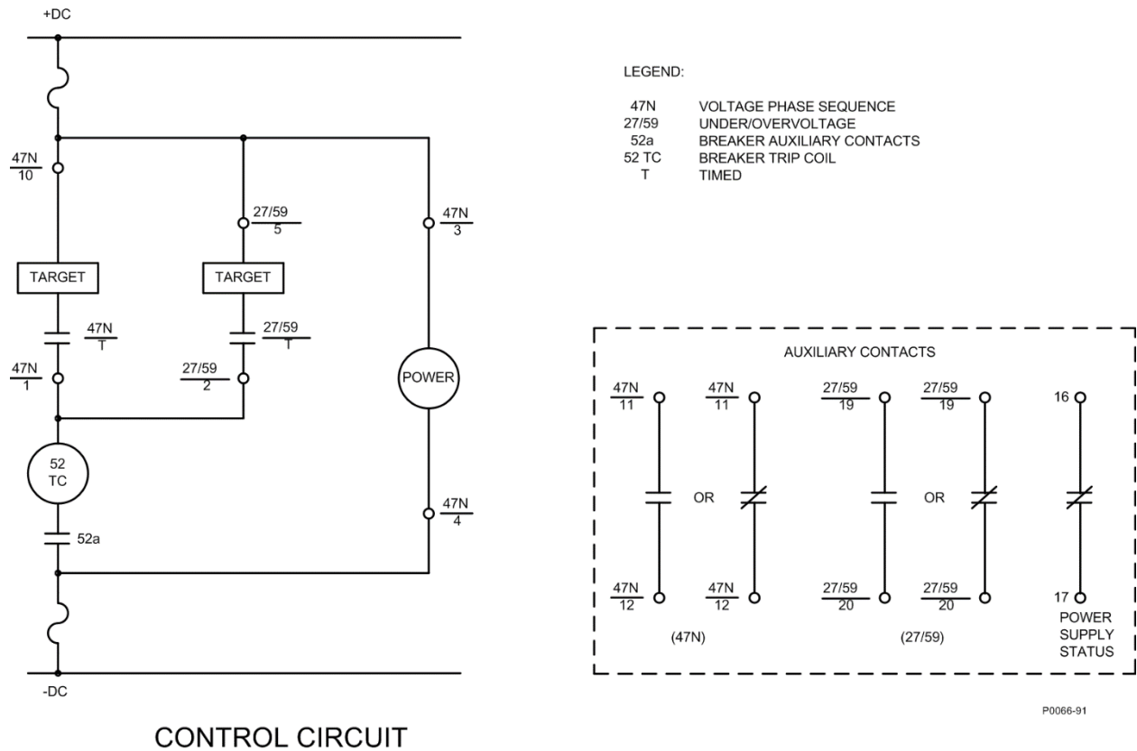
Figure 4-8. Control Circuit Diagram
