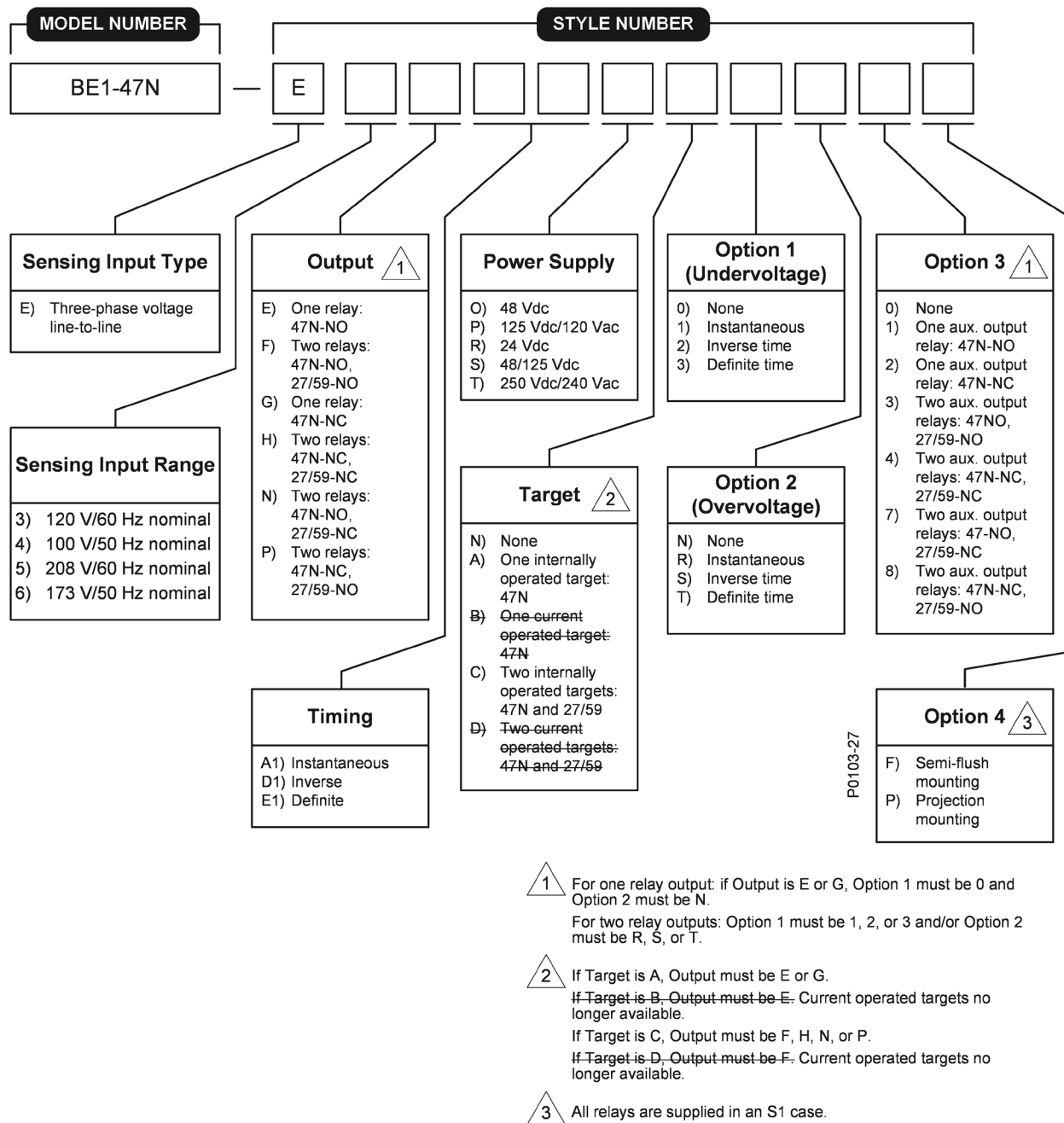
Figure 1-1. BE1-47N Style Identification Chart
