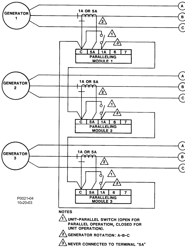
Figure 5. Reactive Differential Compensation, CT Interconnection, 5 A Sensing
