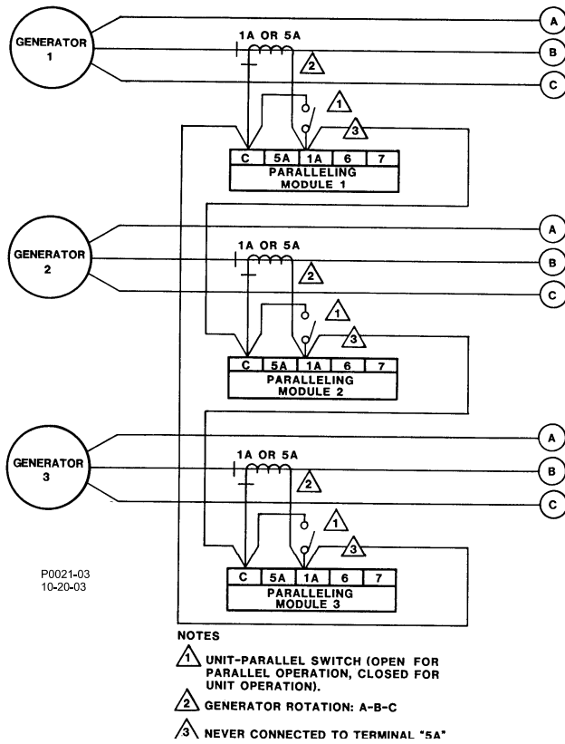
Figure 4. Reactive Differential Compensation, CT Interconnection, 1 A Sensing
