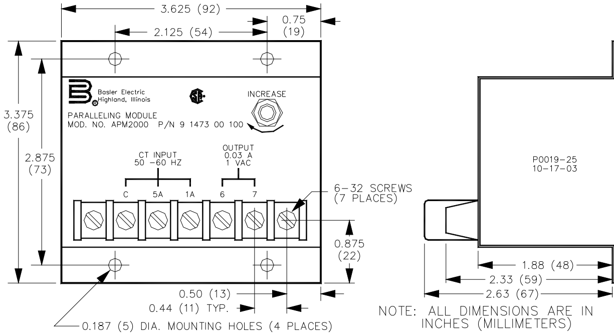
Figure 1. APM 2000 Mounting Dimensions
