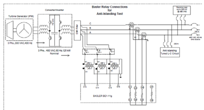
Fig. 3. Testing Grid Loss—External Protection Relay Test Setup
