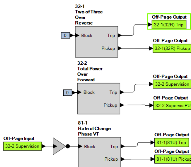
Fig. 7. Power element 32-2 supervised frequency rate-of-change element 81ROC
