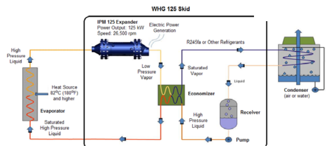
Figure 1. Process diagram shows the flow for the working fluid in the ORC unit
