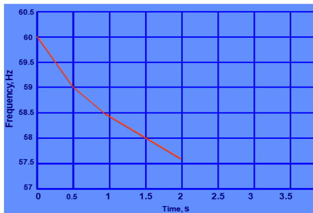
Fig. 6. Utility loss loads DG—frequency declines quickly
