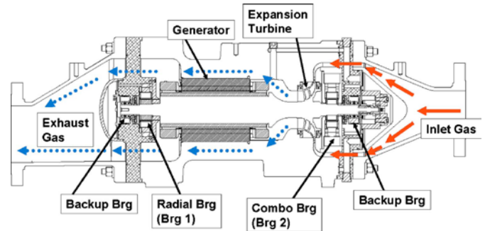
Fig. 2. IPM Cross-section
