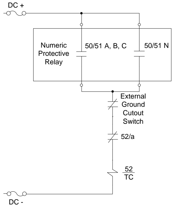
Figure 5: Miswired Simple Overcurrent Scheme
