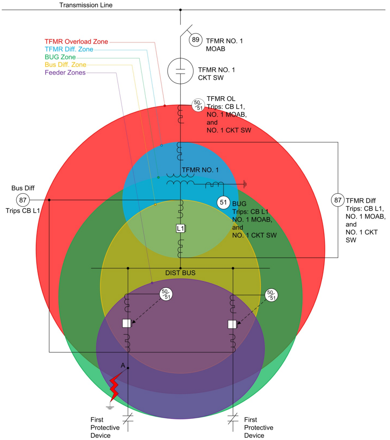
Figure 1: Zones of Protection
