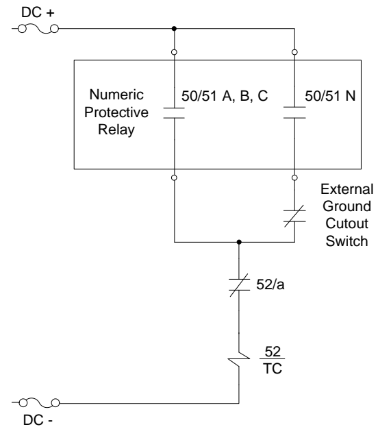
Figure 4: Simple Overcurrent Scheme
