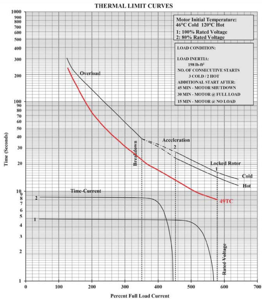
Figure 3: Motor Thermal Limit vs. Programmed 49TC
