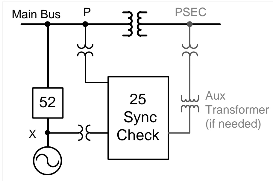
Fig. 7 Typical Sync-Check Connections
