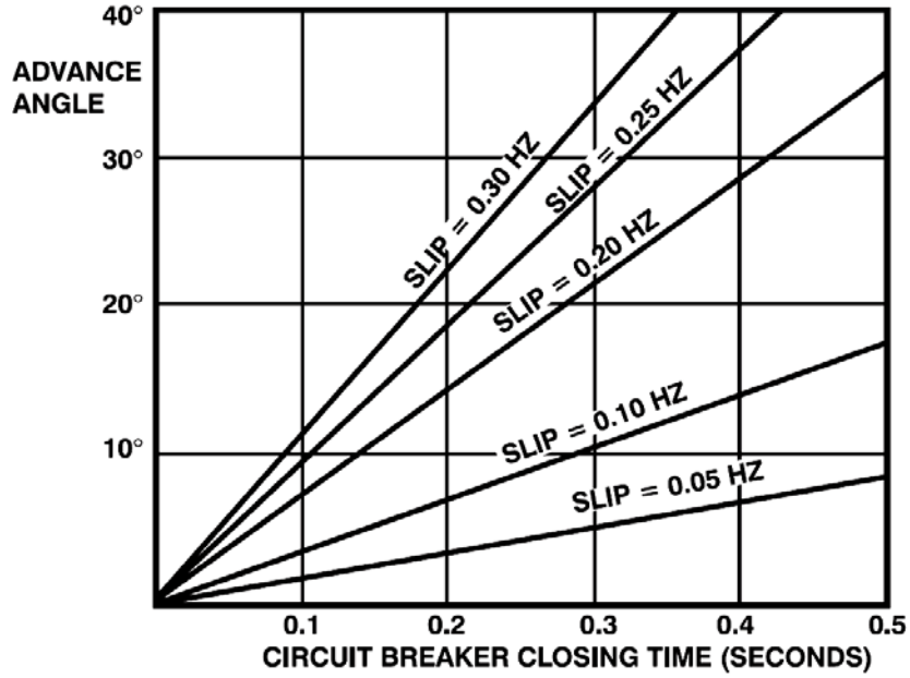
Fig. 5 Sync-Check Closing Quantities
