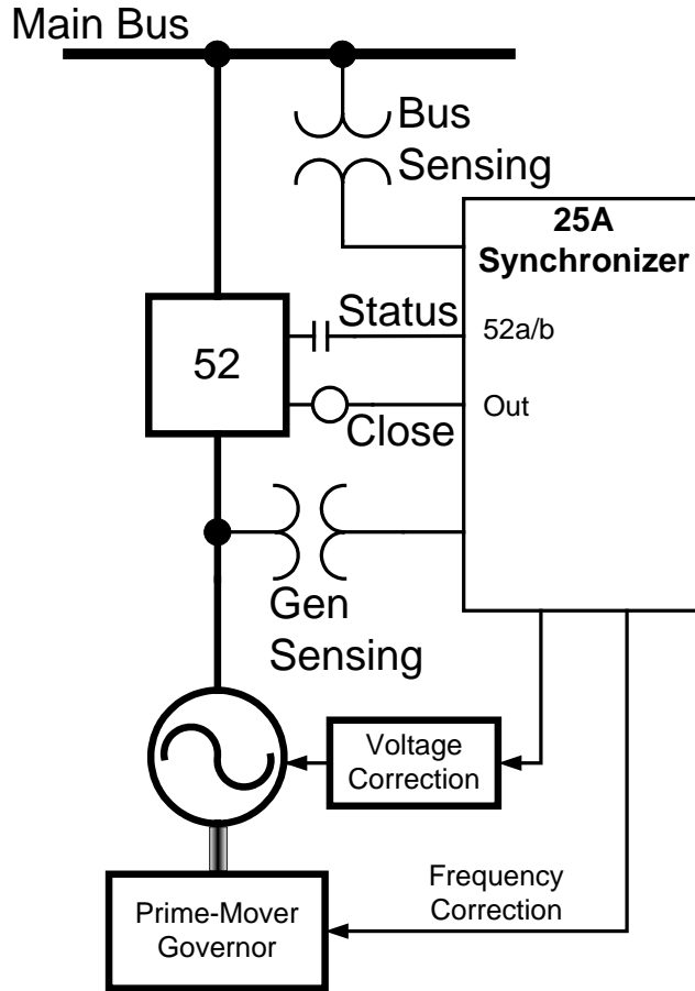
Fig. 4 Synchronizer Connection Diagram
