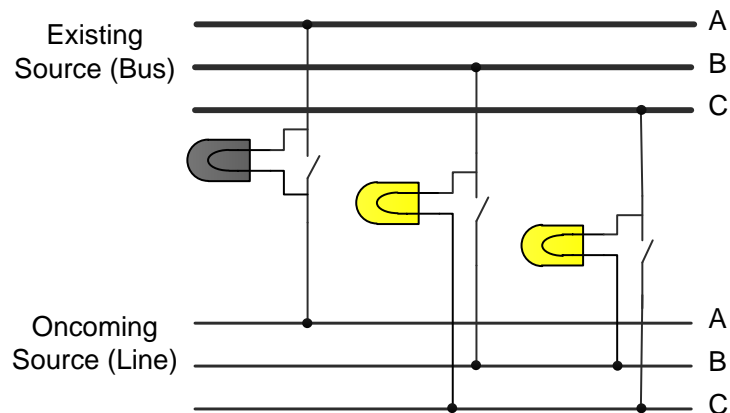
Fig. 2b Two-Bright, One-Dark Lamp
