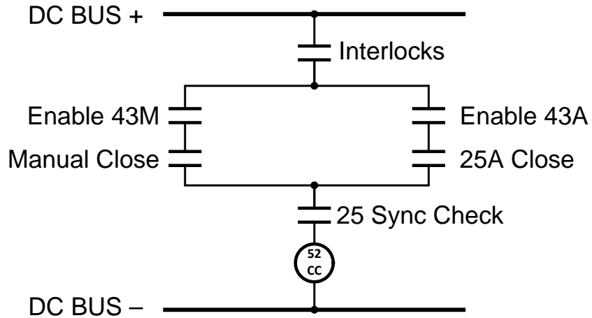
Fig. 6 Supervise Autosynchronizer (25A) with Sync Check (25)
