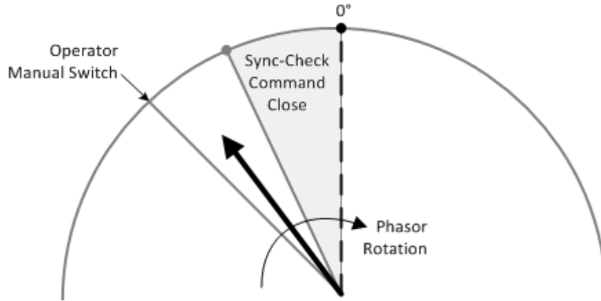
Fig. 3 Assisted-Manual Synchronization with Sync Check
