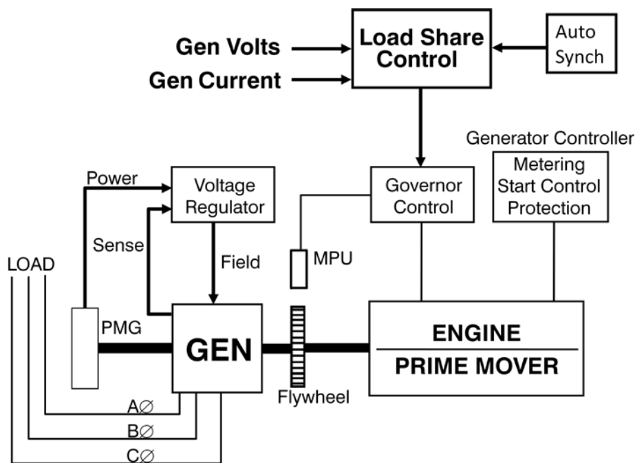
Figure 30: Paralleled System Controls
