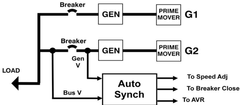
Figure 27: Addition of Auto Synchronizing
