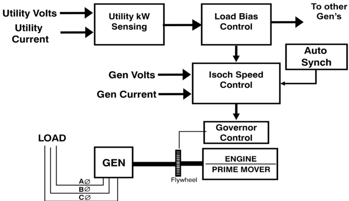
Figure 40: Load control for peak shaving
