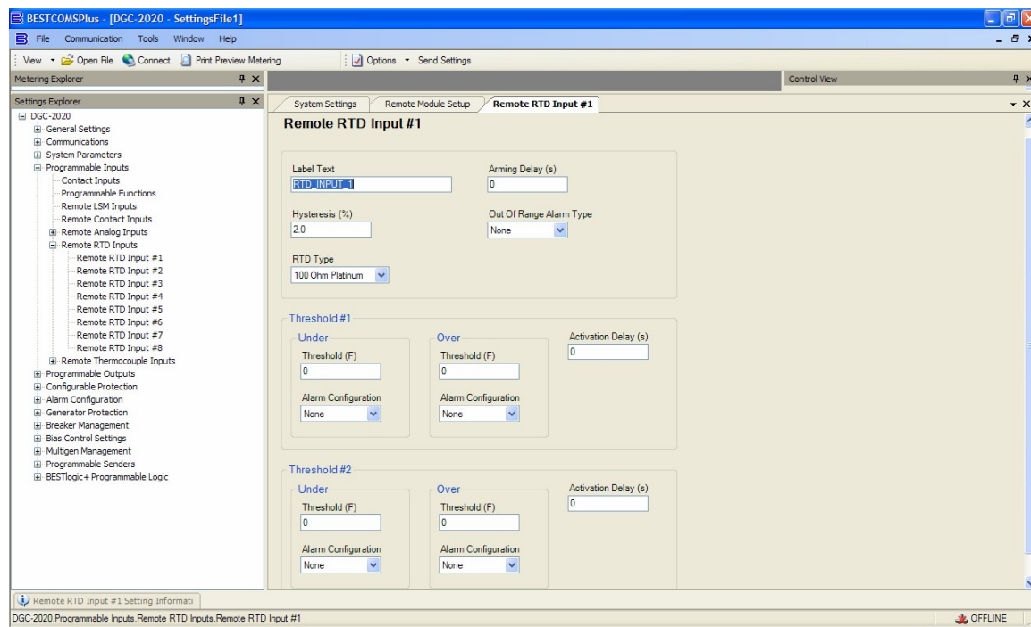
Figure 11: AEM-2020 Configuration Screen
