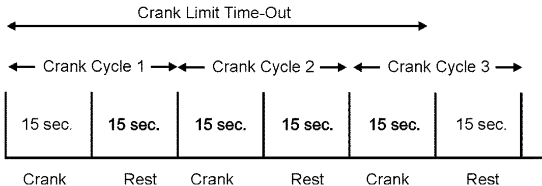
Figure 6: Crank/Rest Cycles
