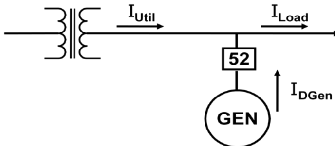
Figure 49: Generator kW shared with utility
