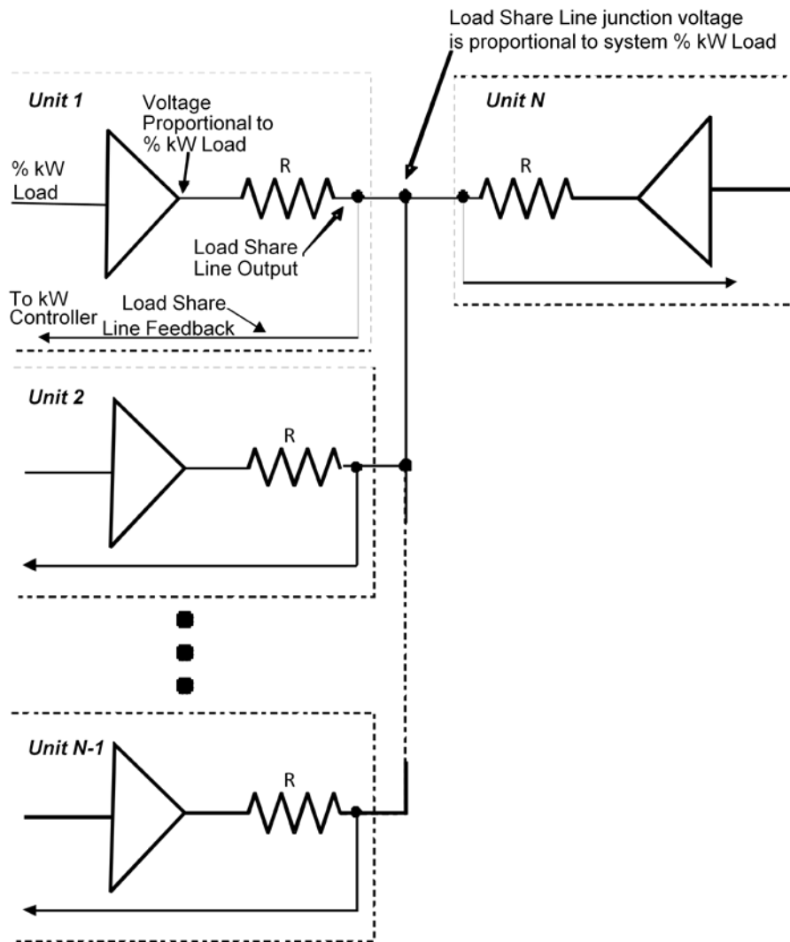
Figure 33: A Load Share Line Implementation on a System of N Machines
