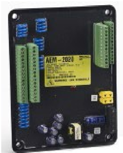
Figure 9: AEM-2020 (Analog Expansion Module)
