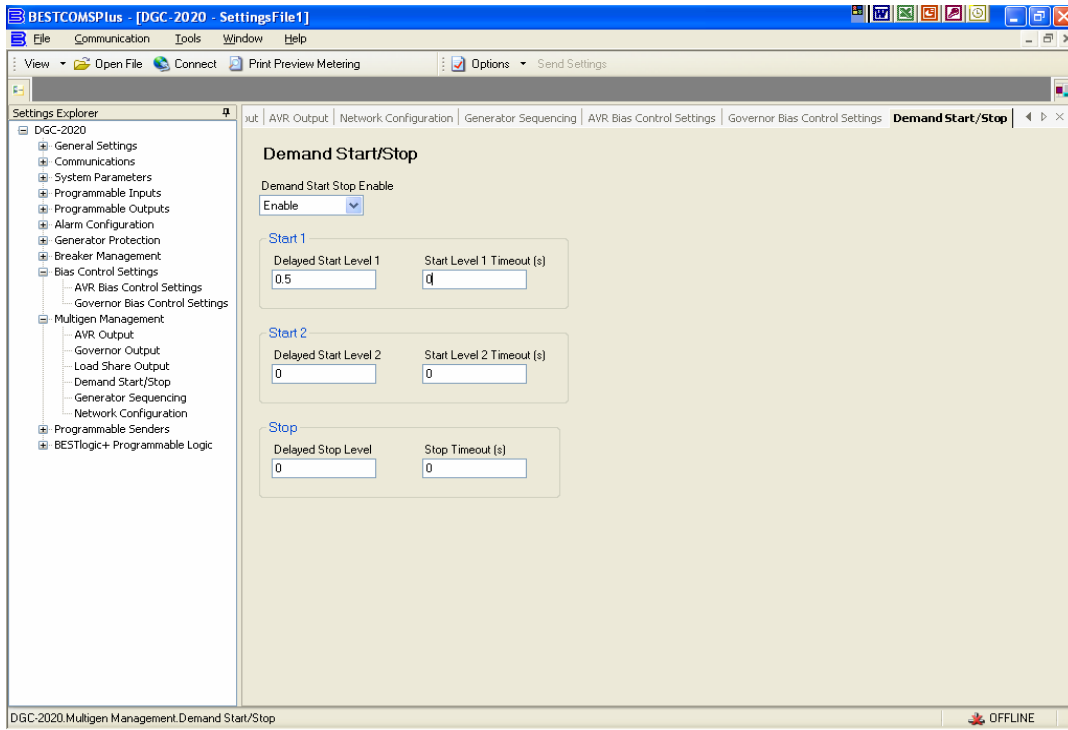
Figure 52: Demand Start/Stop (BESTCOMSPiUs®)
