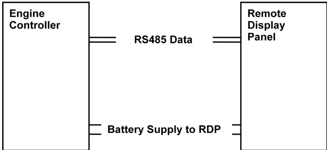
Figure 15: Communications Remote Display for NFPA 110
