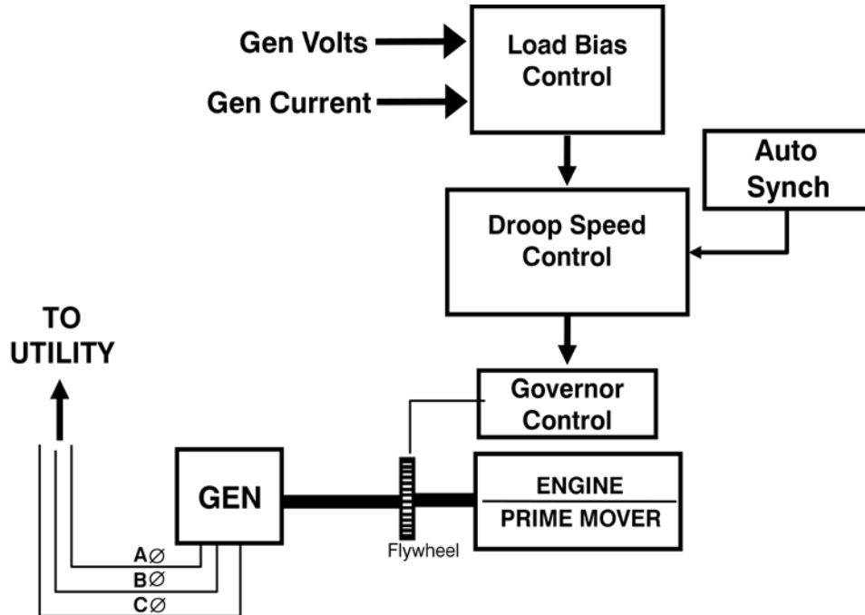
Figure 38: Isochronous Governor Controls to Base Load to Utility
