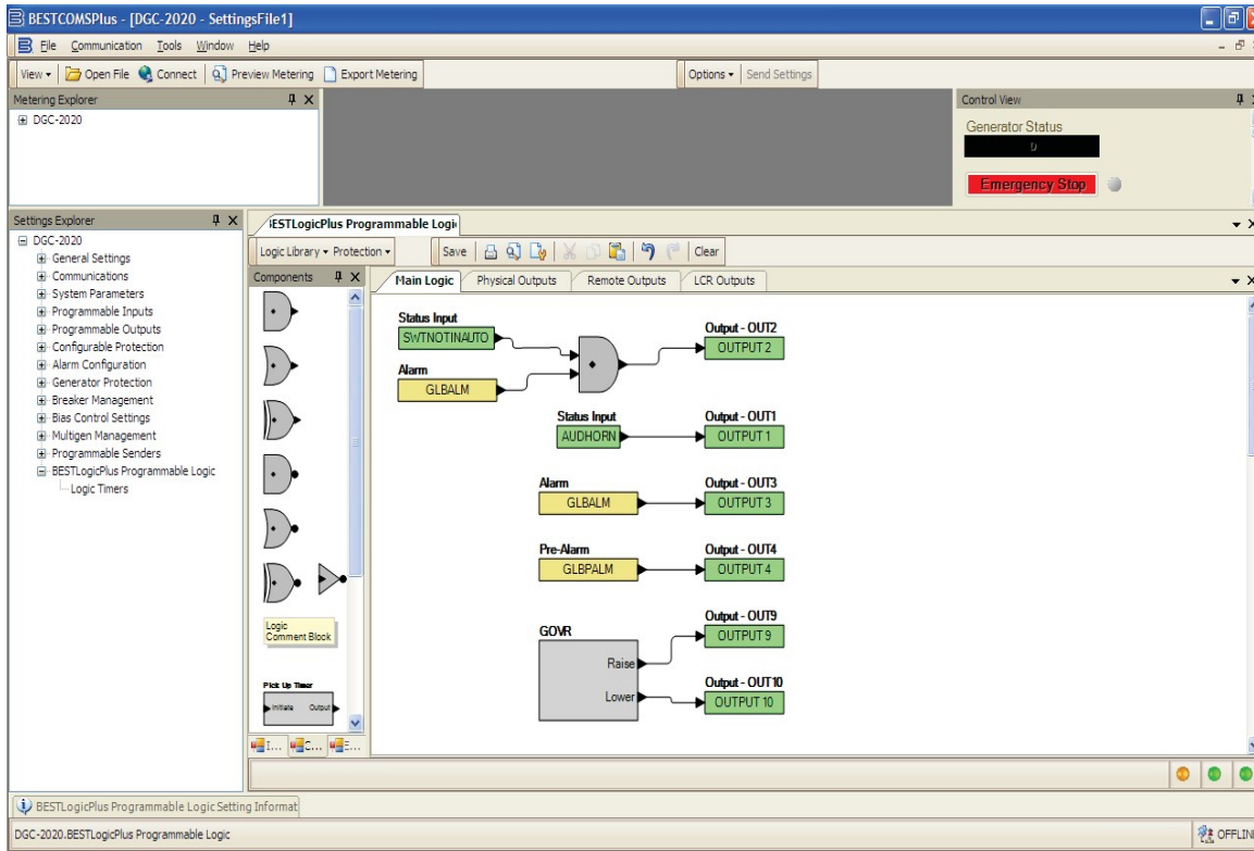
Figure 13: DGC-2020 Programmable Logic
