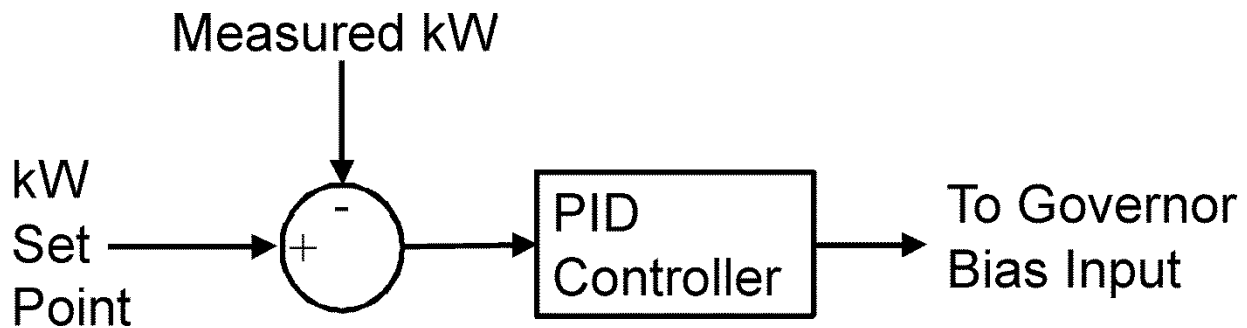
Figure 32: kW Controller Block Diagram
