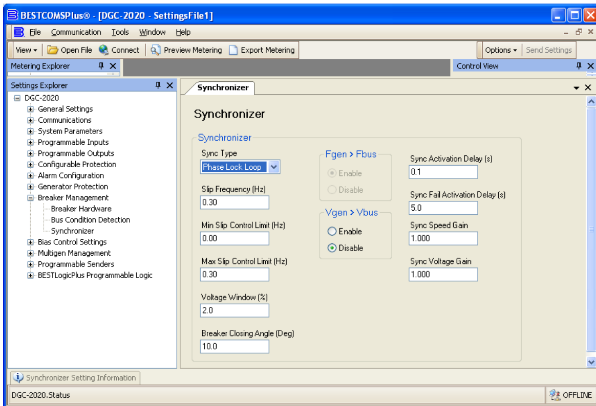
Figure 28: Synchronizer Settings (BESTCOMSPPlus®)
