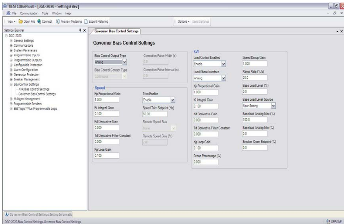
Figure 43: Load Ramping On/Off - Ramp Rate % Settings (BESTCOMS™)
