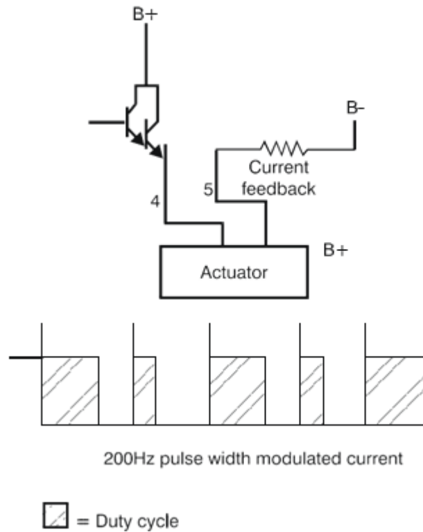
Figure 25: Actuator Drive Output
