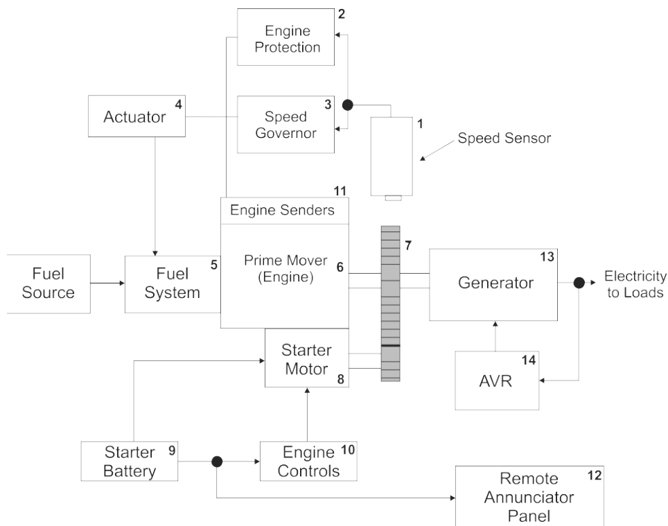
Figure 1: Typical Genset Block Diagram
