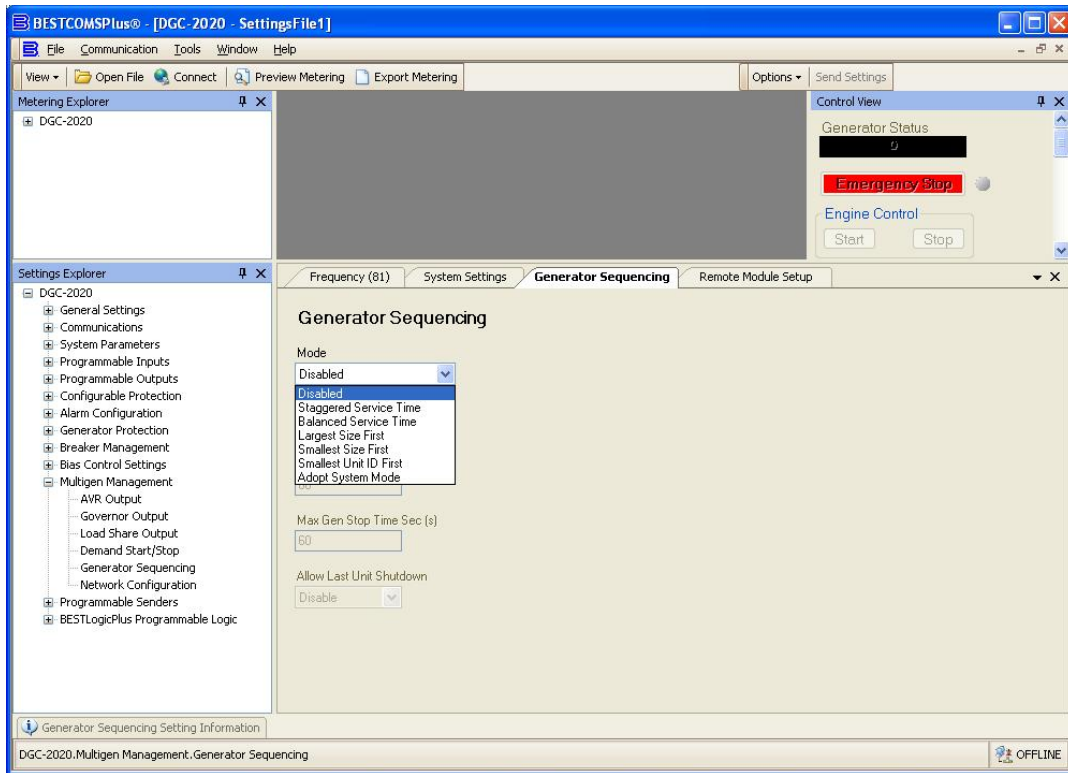
Figure 53: Generator Sequencing Settings, Mode Selection (BESTCOMSPiUs®)
