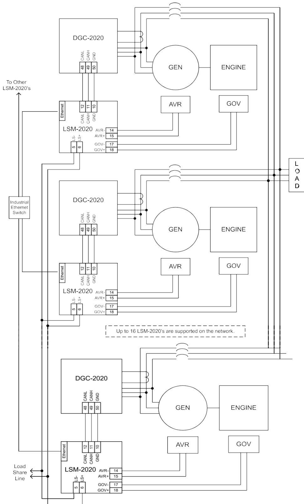
Figure 34: Typical load sharing interconnection
