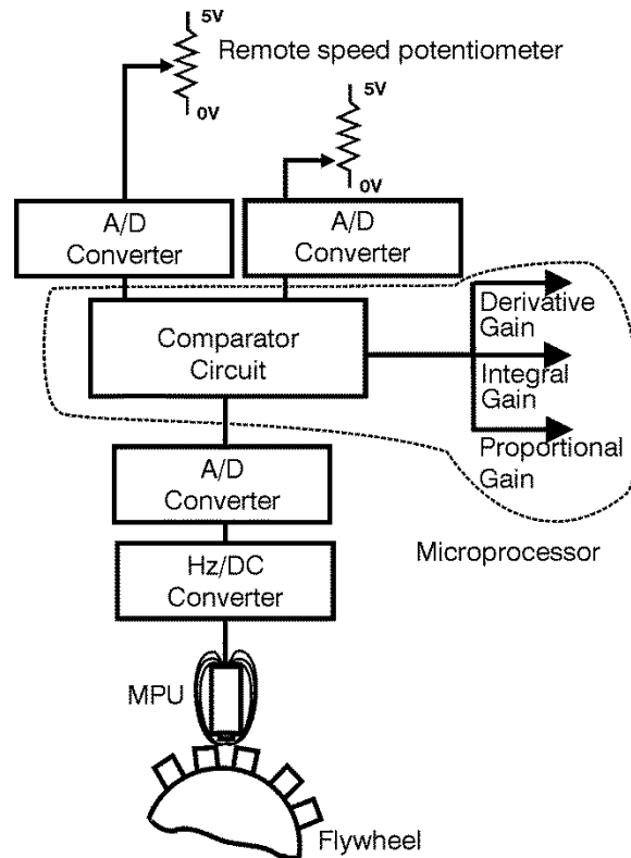
Figure 24: PID Gain Circuits in Governor
