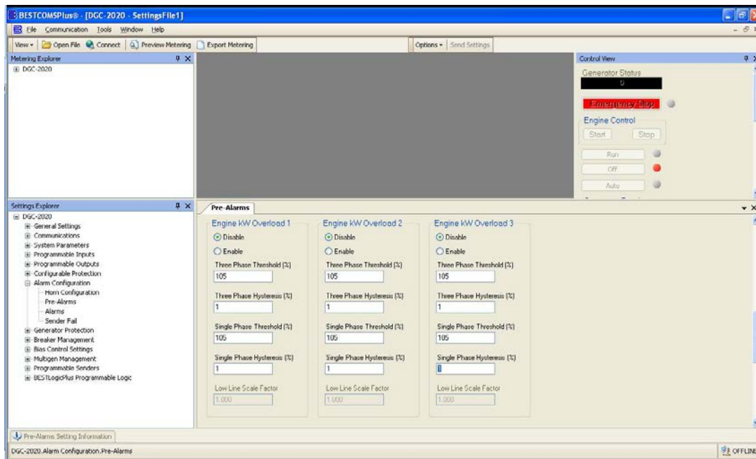
Figure 47: kW Overload Settings (BESTCOMSPPlus®)
