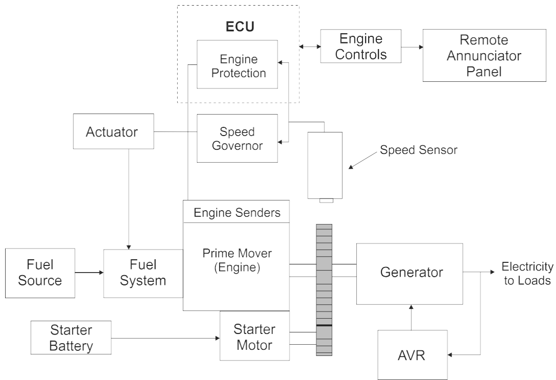
Figure 17: Typical Genset with ECU Equipped Engine
