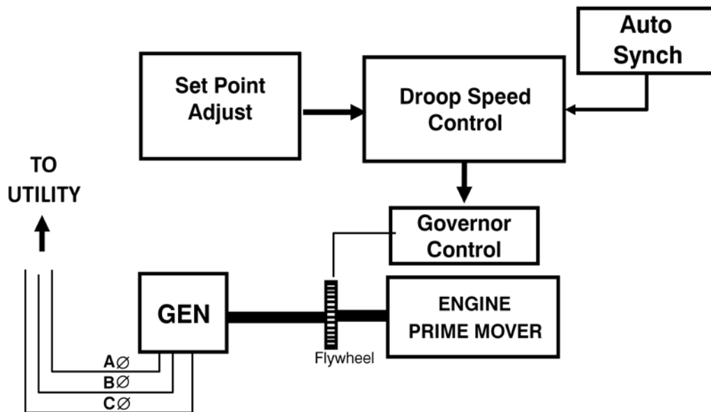
Figure 37: Droop Governor Controls to Base Load to Utility
