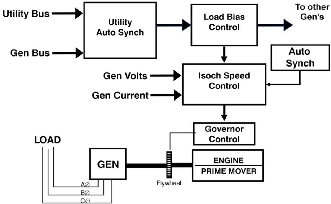
Figure 41: Synchronize to Utility with Multiple Generators
