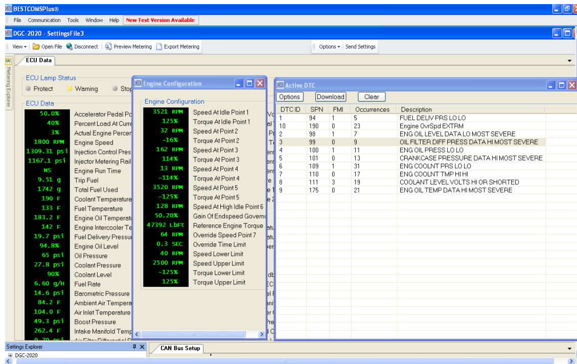
Figure 21: Typical PC Screen Showing DTC Information
