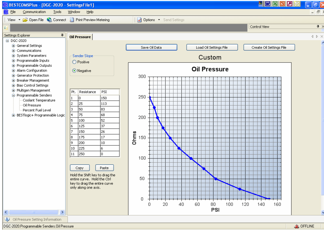
Figure 5: Programmable Sender Curves
