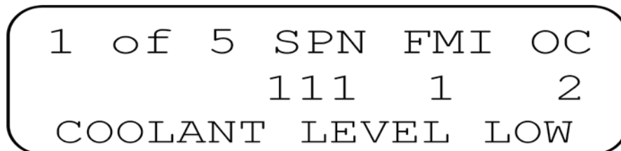
Figure 20: Typical DGC Front Panel DTC Display
