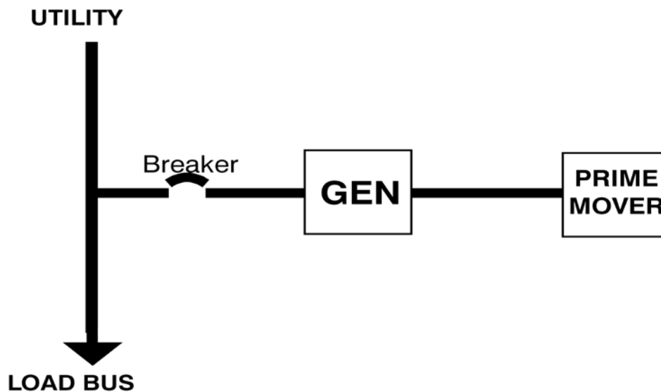
Figure 36: Generator in Parallel with Infinite Utility Bus
