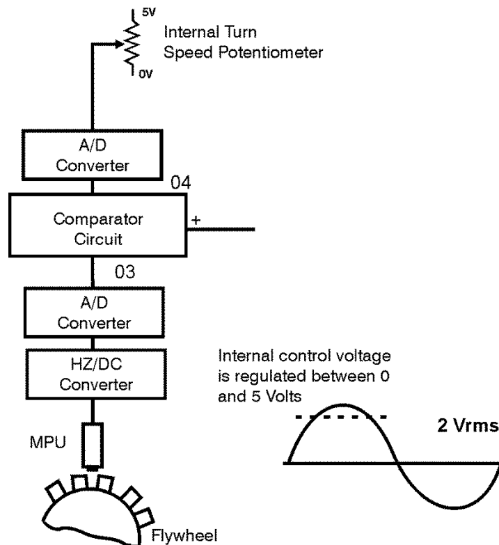
Figure 3: Speed Input to the Comparator
