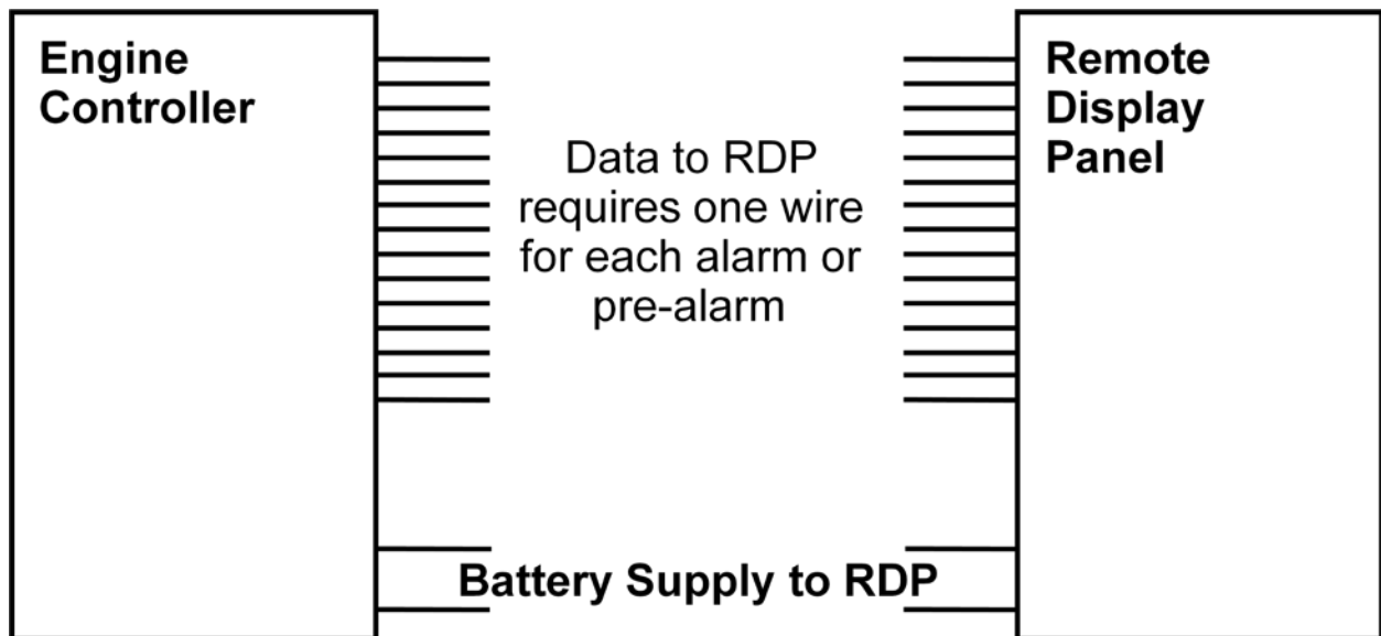
Figure 14: Conventional Remote Display for NFPA 110
