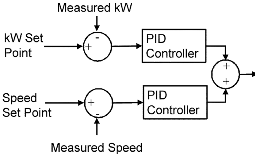
Figure 35: Controller Implementation with kW Controller and Speed Trim Controller
