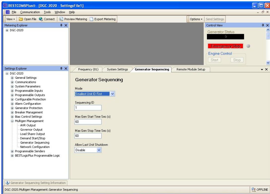
Figure 54: Generator Sequencing Settings Screen (BESTCOMSPlus®)
