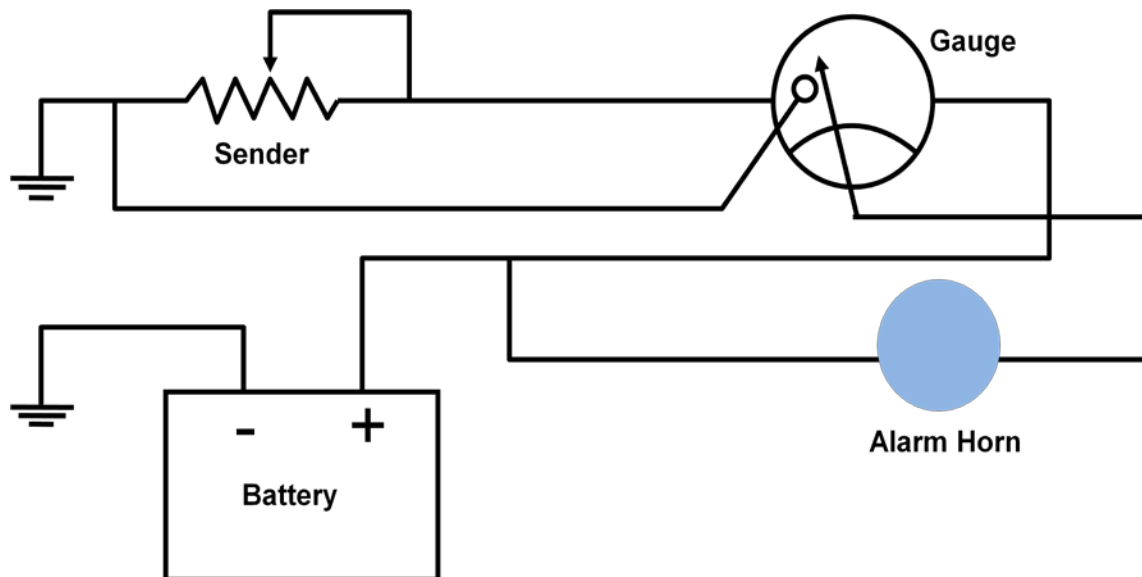
Figure 7: Gauge with an internal switch
