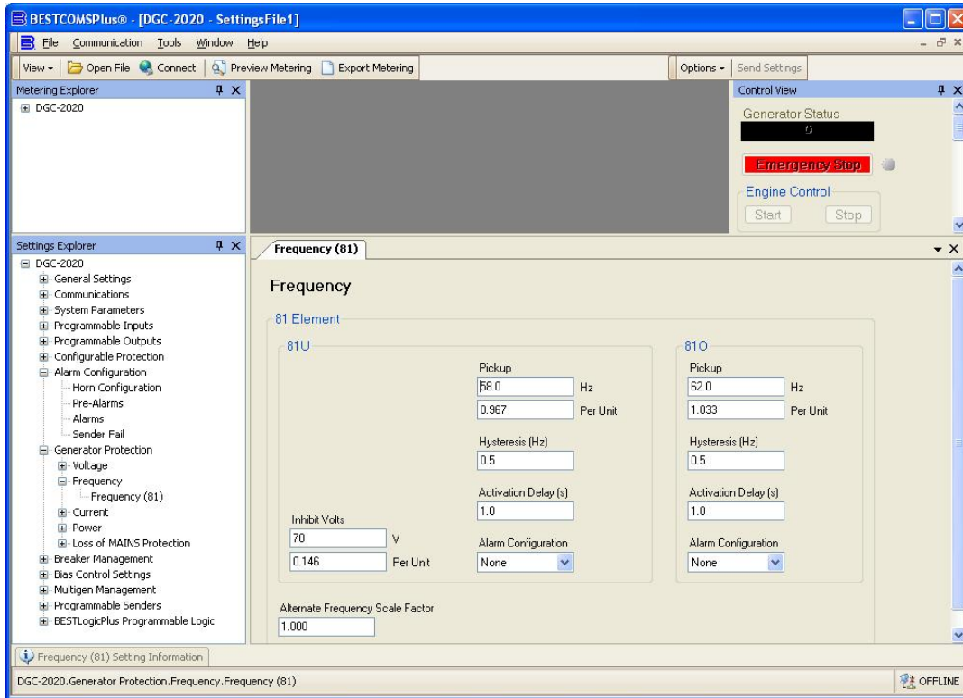
Figure 48: Underfrequency Protection Settings BESTCOMSPPlus®)
