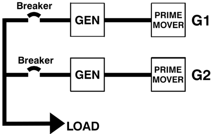
Figure 26: Islanded Generator Bus
