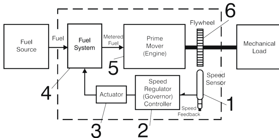
Figure 23: Speed Control Loop
