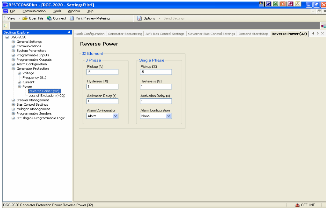
Figure 51: Reverse power protection (BESTCOMSPPlus®)
