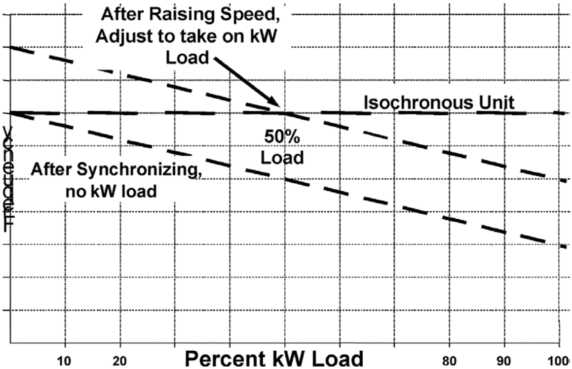
Figure 31: Speed Droop Characteristic
