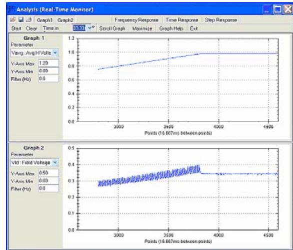
Figure 9: Voltage Buildup in Voltage Regulator Mode
