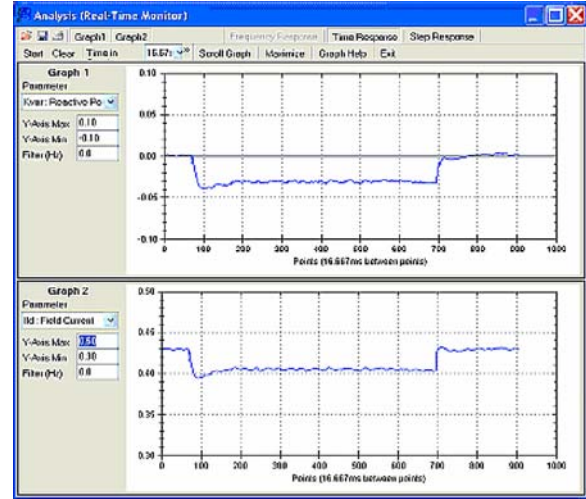
Figure 11: Under Excitation Limit Dynamic Step Test
