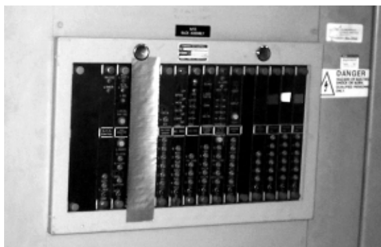
Figure 1: GE Bus Fed Analog Voltage Regulator
