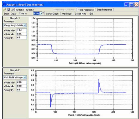
Figure 10: 5% Voltage Step Change in Voltage Regulator Mode
