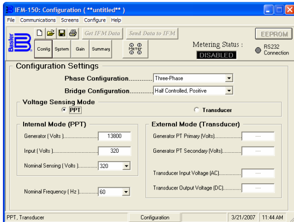
Figure 8: Firing Circuit setup for Half-Wave Bridge
