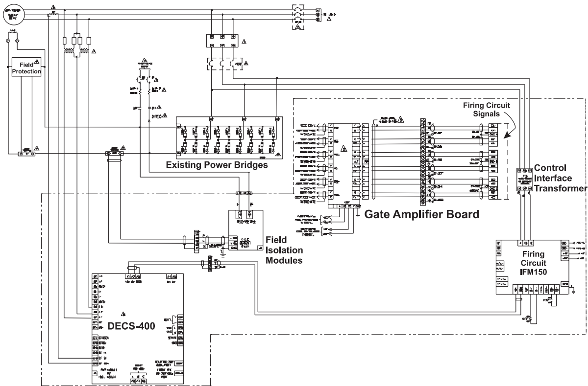
Figure 7: Partial schematic of the new interconnected system
