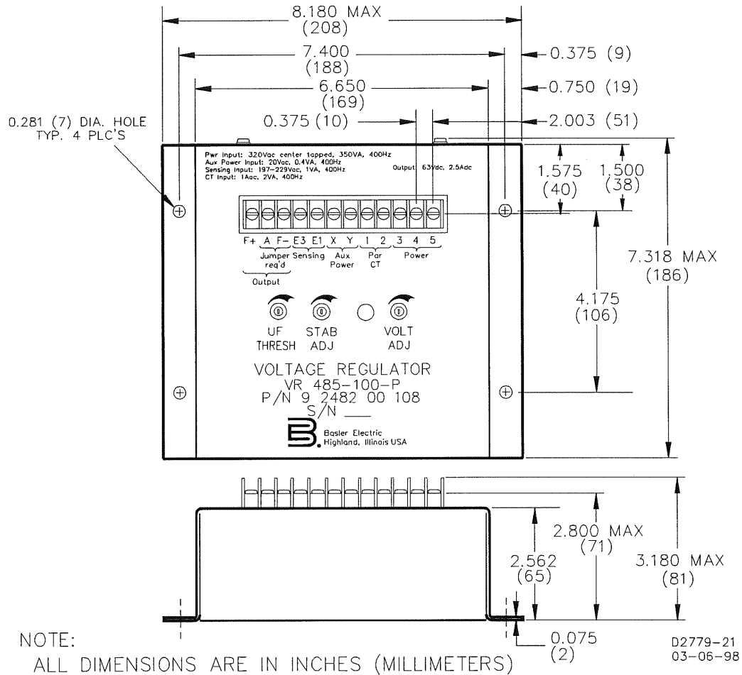
Figure 2-1. Outline Drawing
