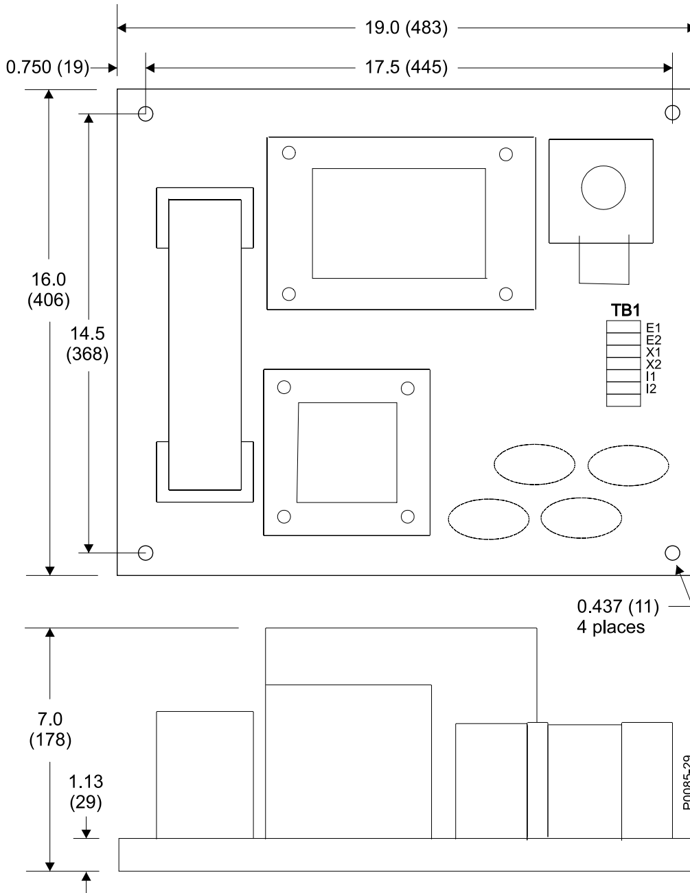
Figure 3. SBO Chassis Dimensions
