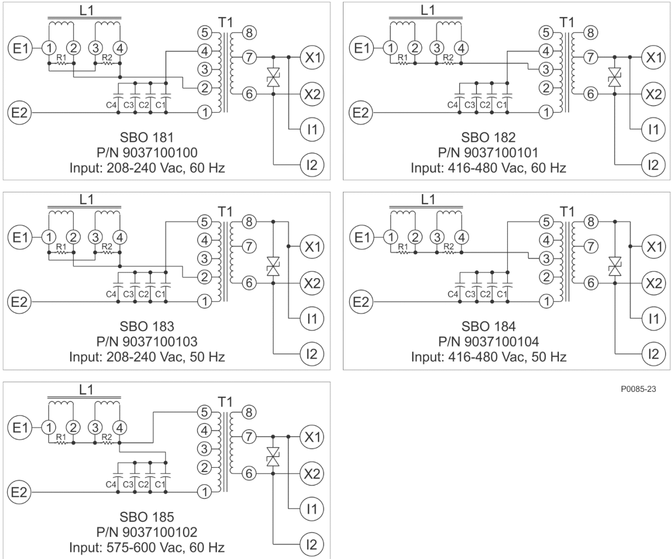
Figure 6. Schematic Diagrams, Reservoir Assemblies
