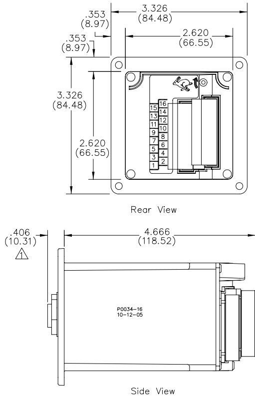
Figure 2. DGC-50 Overall Dimensions
