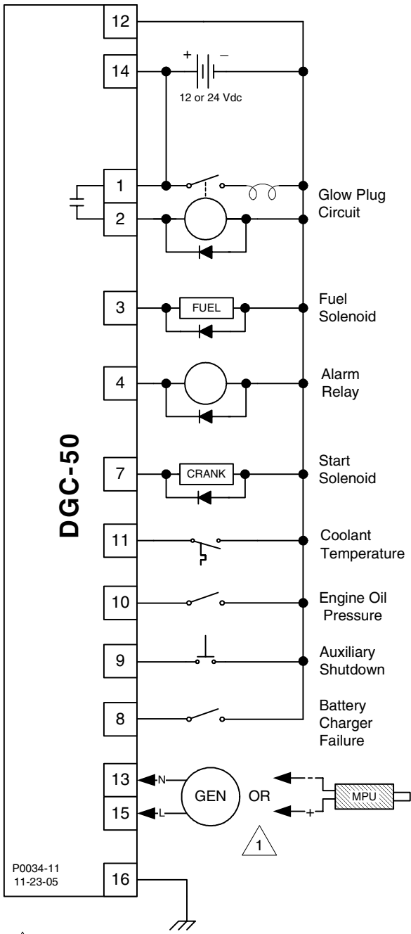
Figure 6. Typical Connections, Style XL
