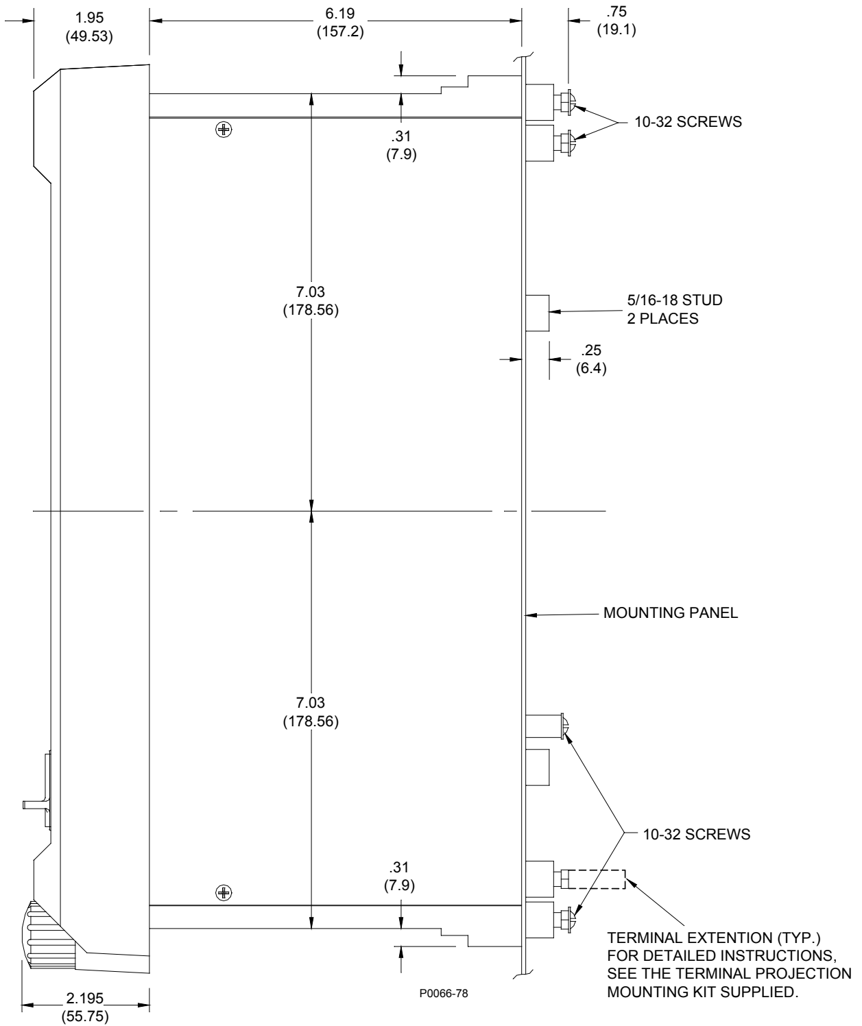
Figure 4-6. M1 Case Dimensions, Side View, Double Ended, Projection Mount
