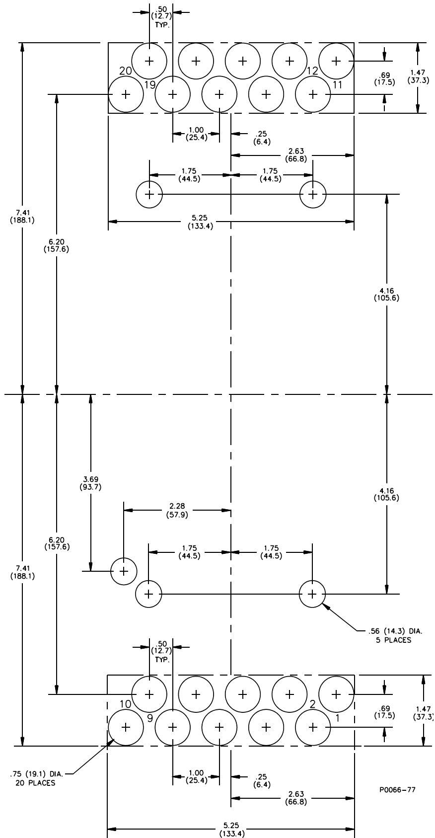
Figure 4-4. Panel Cutting/Drilling, Double Ended, Projection Mount Case
