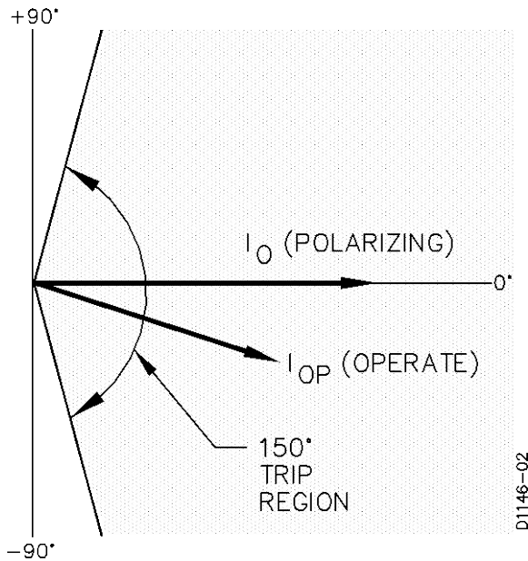
Figure 3-2. Zero Sequence Current Polarizing Phase Relationship
