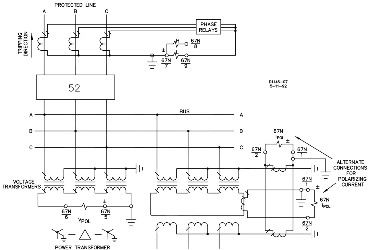
Figure 4-10. Typical Sensing Input Connections (Three Winding Transformer)
