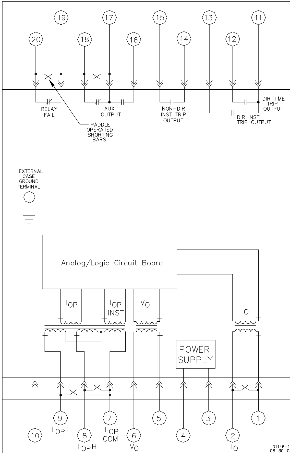
Figure 4-8. Typical Internal Connections
