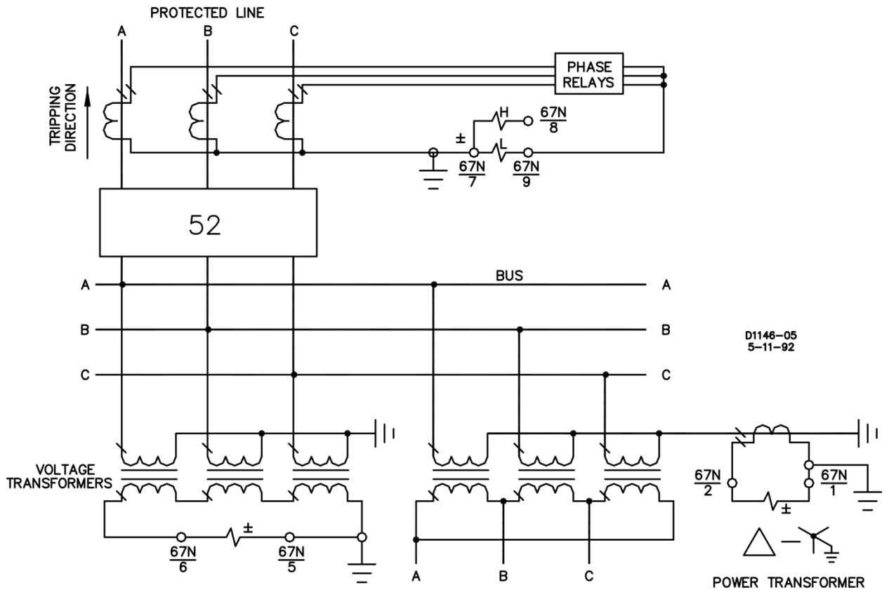
Figure 4-9. Typical Sensing Input Connections (Two Winding Transformer)
