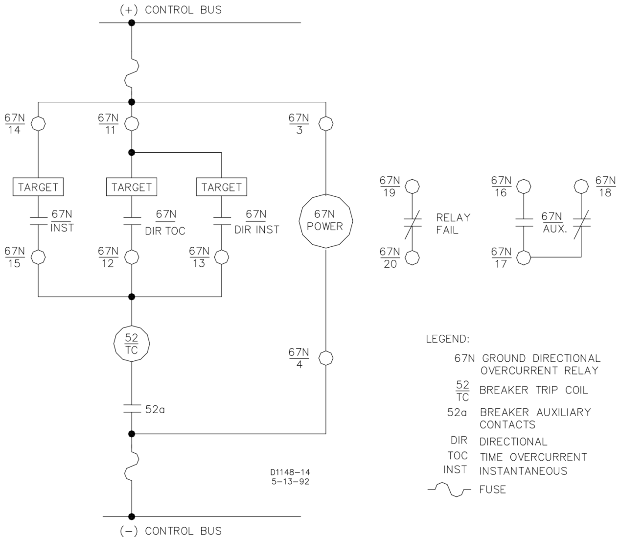
Figure 4-11. Typical Output Connections
