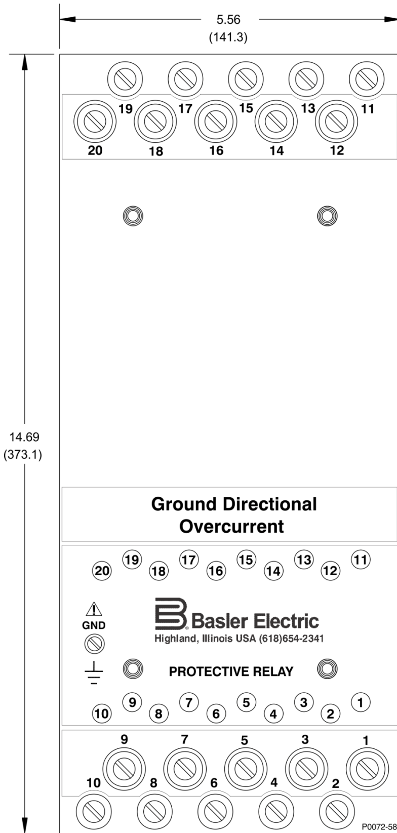
Figure 4-5. M1 Case Dimensions, Rear View, Double Ended, Projection Mount
