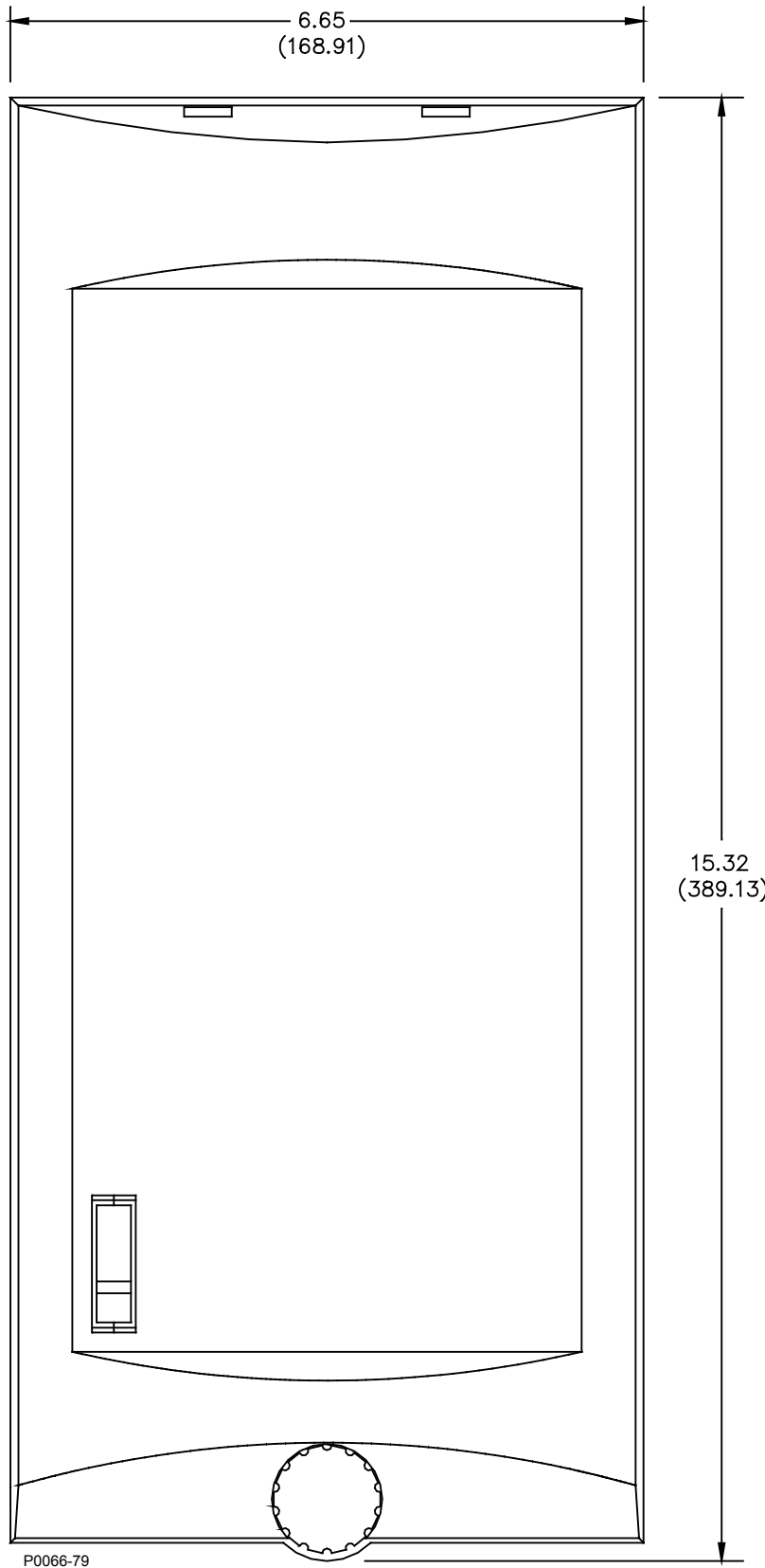
Figure 4-7. M1 Case Cover Dimensions, Front View
