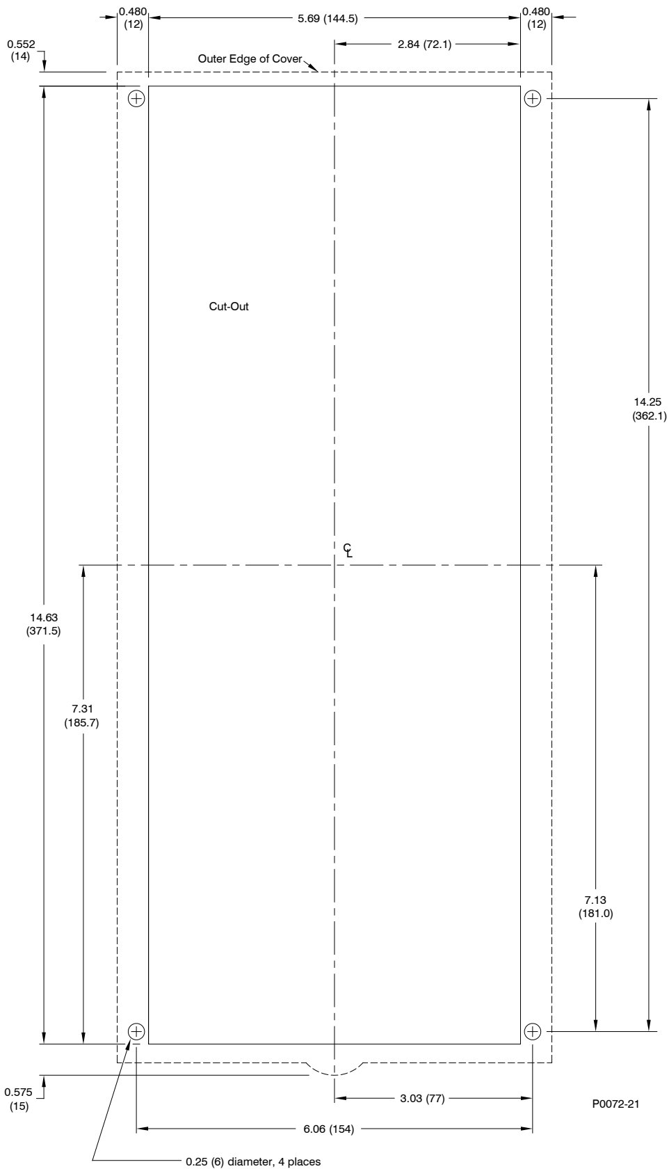
Figure 4-1. Panel Cutting/Drilling, Semi-Flush, M1 Case
