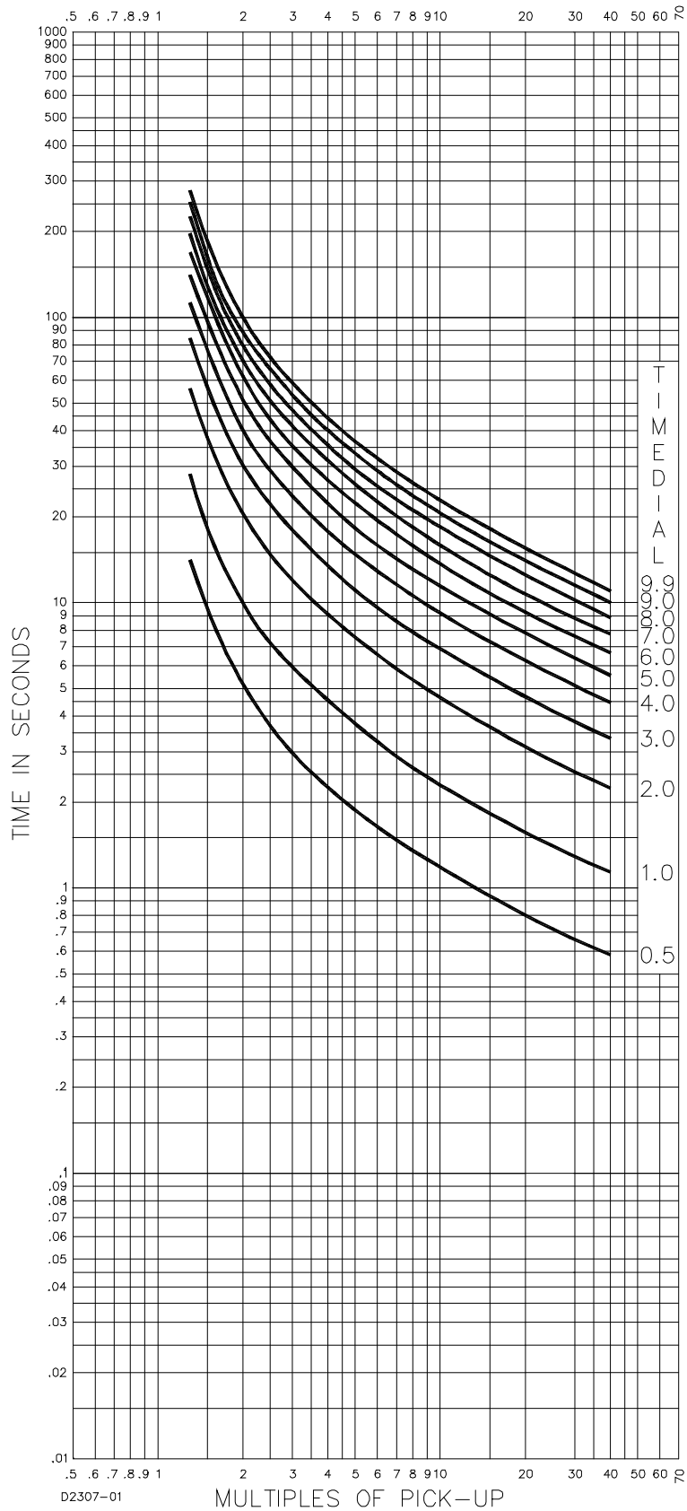
Figure 8-11. Time Characteristic Curve, L2-Long Inverse (SW3-3 ON, Similar to GE IAC 66)
