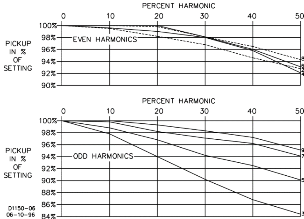
Figure 6-4. Harmonic Rejection
