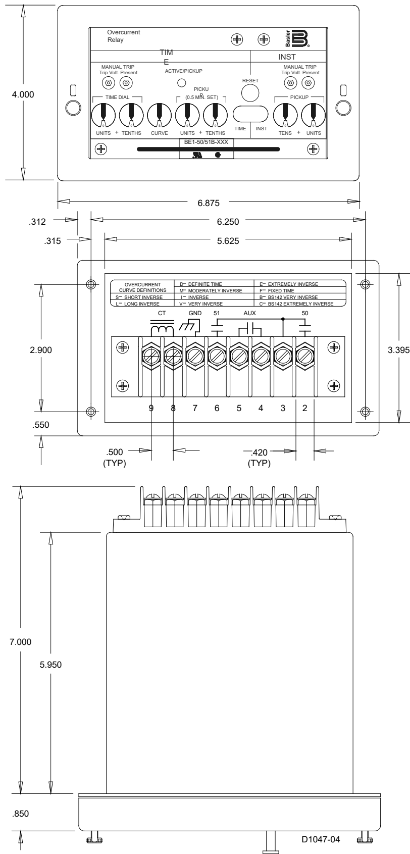
Figure 4-2. Outline Dimensions
