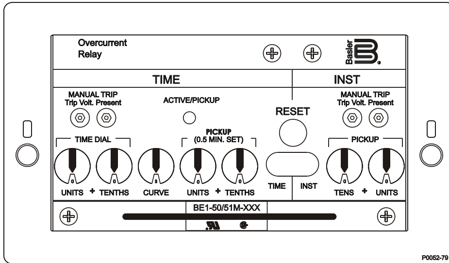
Figure 1-1. BE1-50/51M, C1 Horizontal Mount Case
