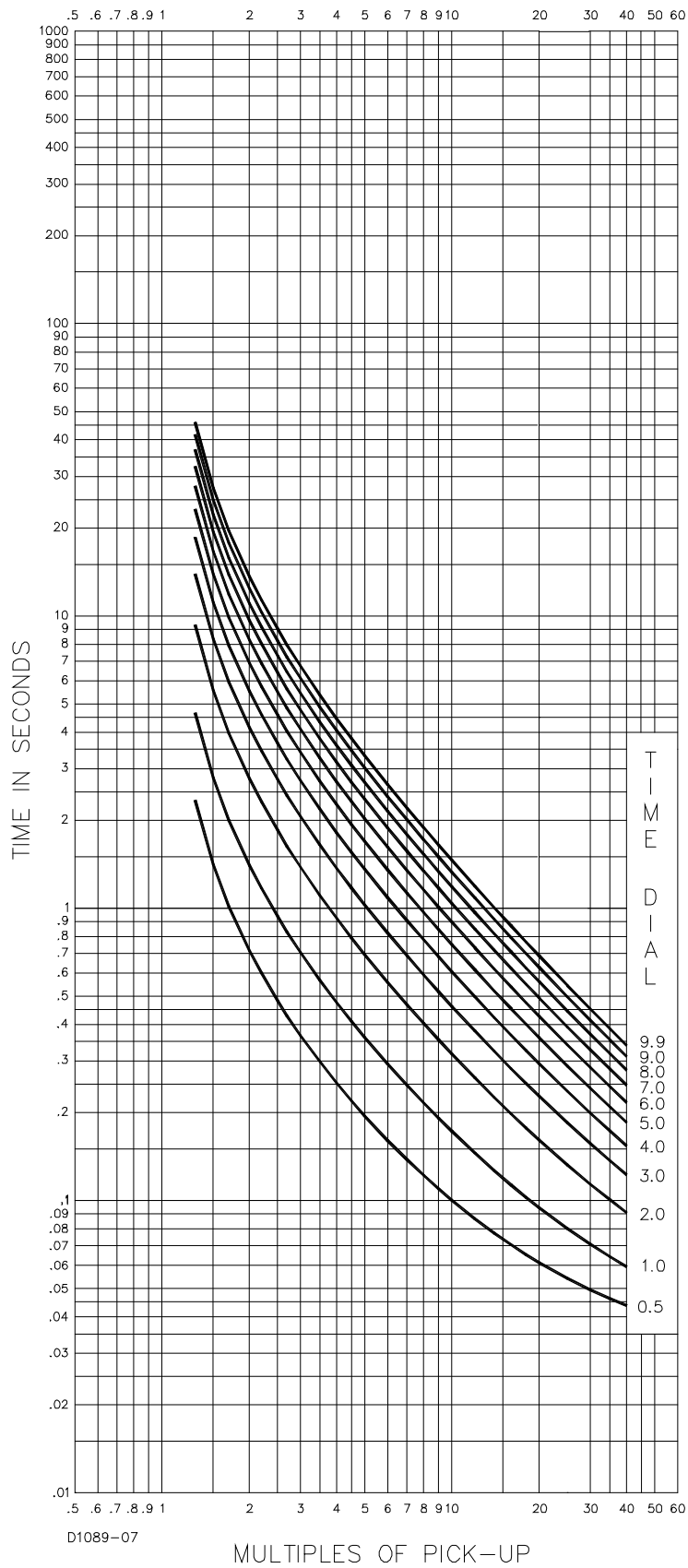
Figure 8-8. Time Characteristic Curve, BS142-B (BS142 Very Inverse)
