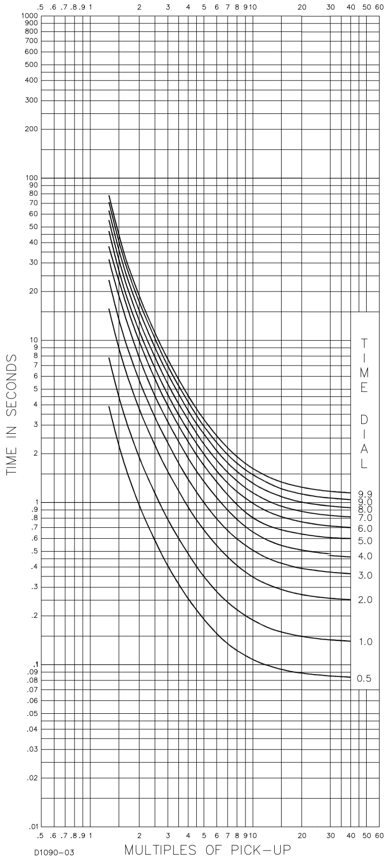
Figure 8-6. Time Characteristic Curve, V-Very Inverse (SW3-3 OFF, Similar to ABB CO-9)
