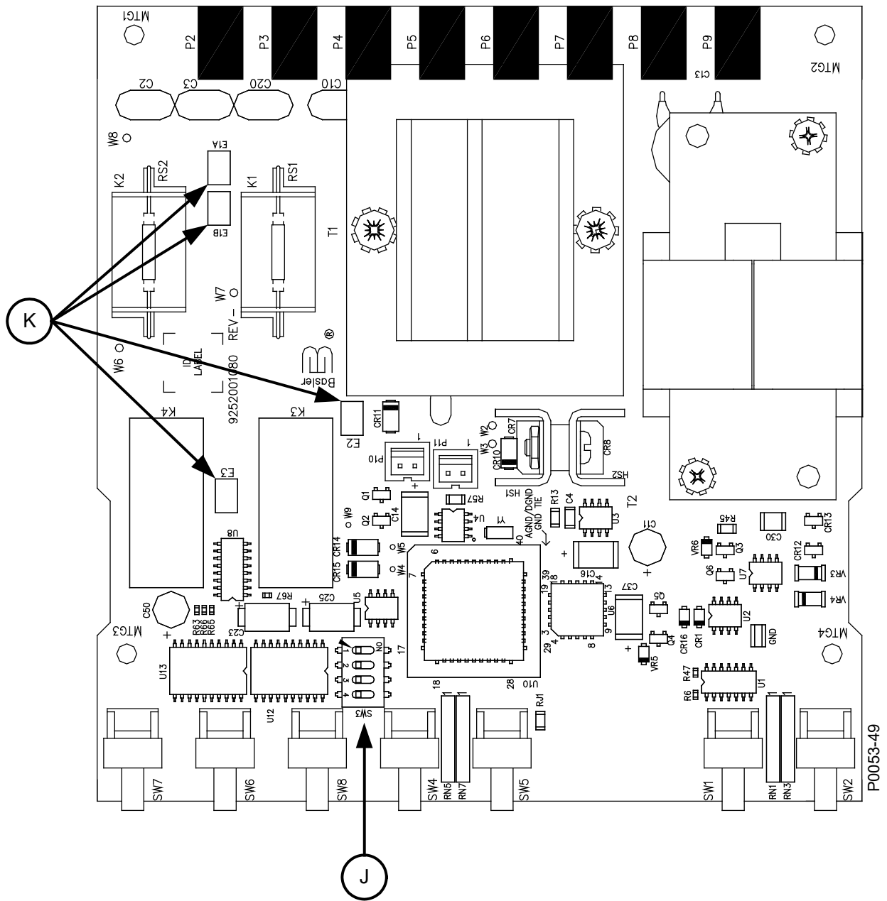
Figure 7-1. Location of SW3 and Auxiliary Output Jumper Terminations
