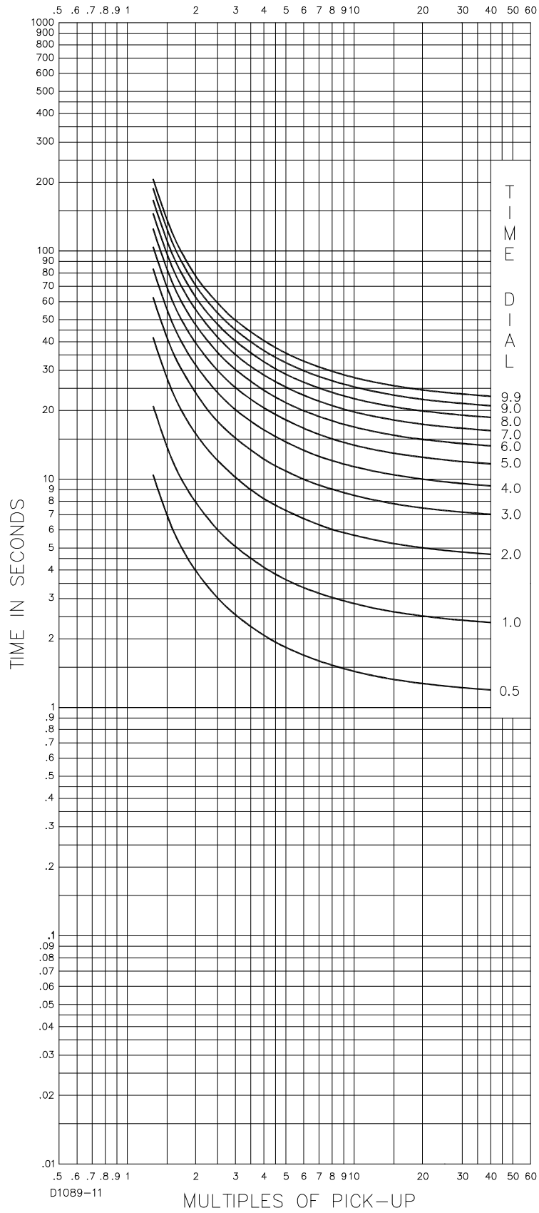
Figure 8-2. Time Characteristic Curve, L-Long Inverse (SW3-3 OFF, Similar to ABB CO-5)
