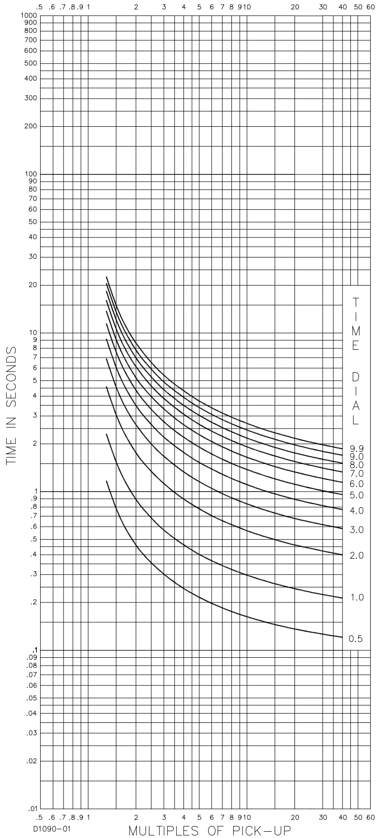
Figure 8-4. Time Characteristic Curve, M-Moderately Inverse (Similar to ABB CO-7)
