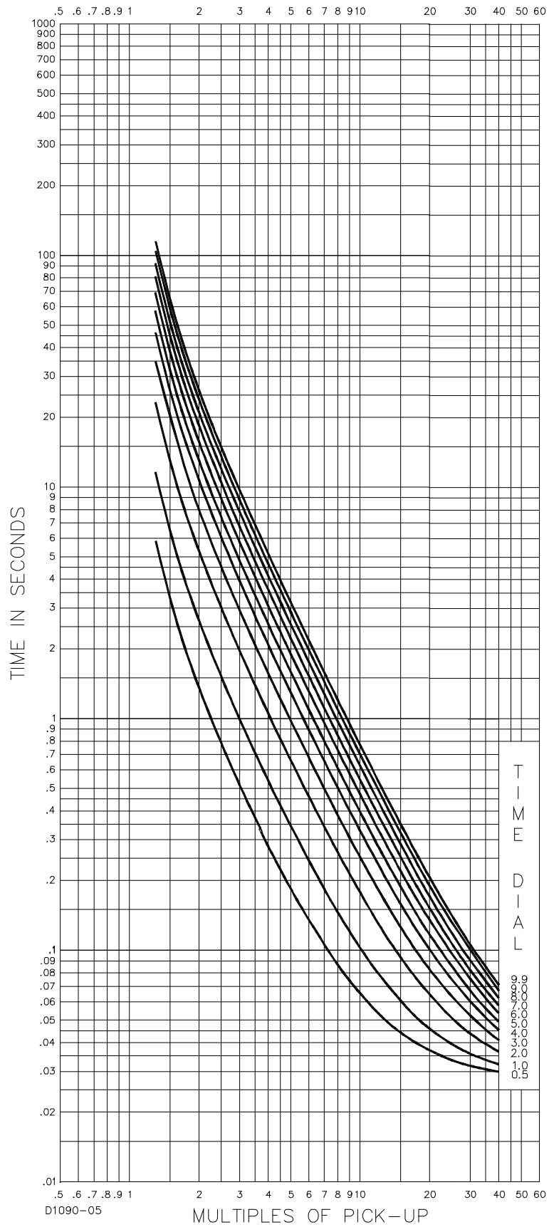
Figure 8-9. Time Characteristic Curve, BS142-C (BS142 Extremely Inverse)
