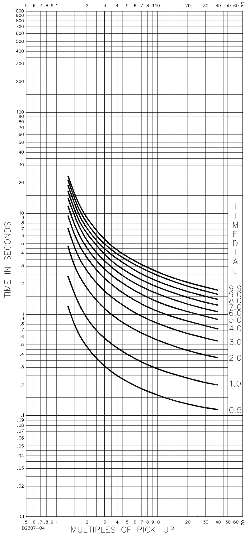
Figure 8-12. Time Characteristic Curve, I2-Inverse (SW3-3 ON, Similar to GE IAC 51)
