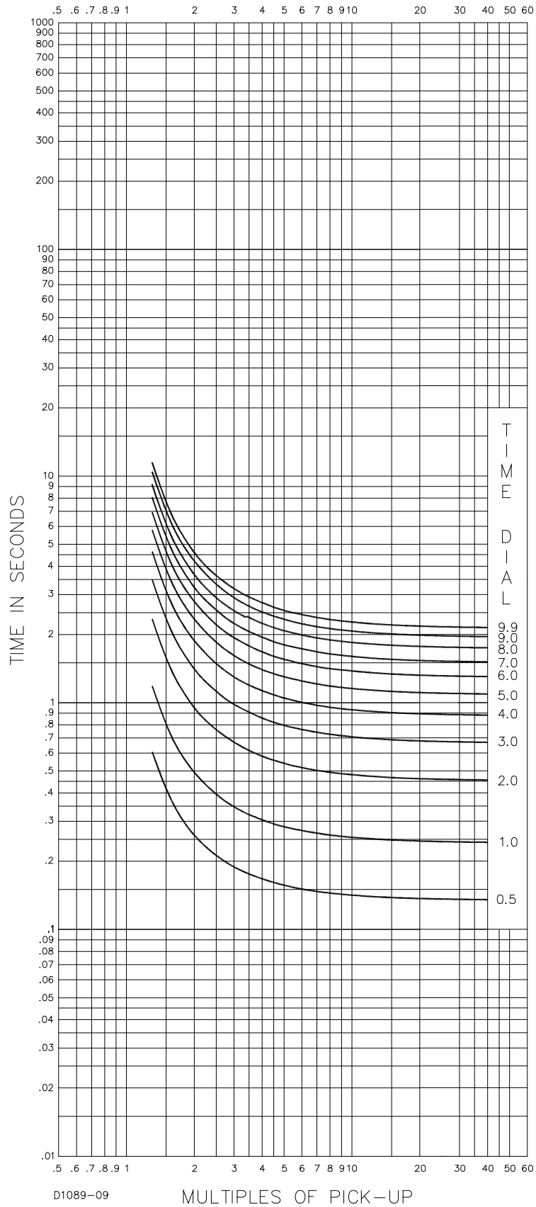
Figure 8-3. Time Characteristic Curve, D-Definite Time (Similar to ABB CO-6)
