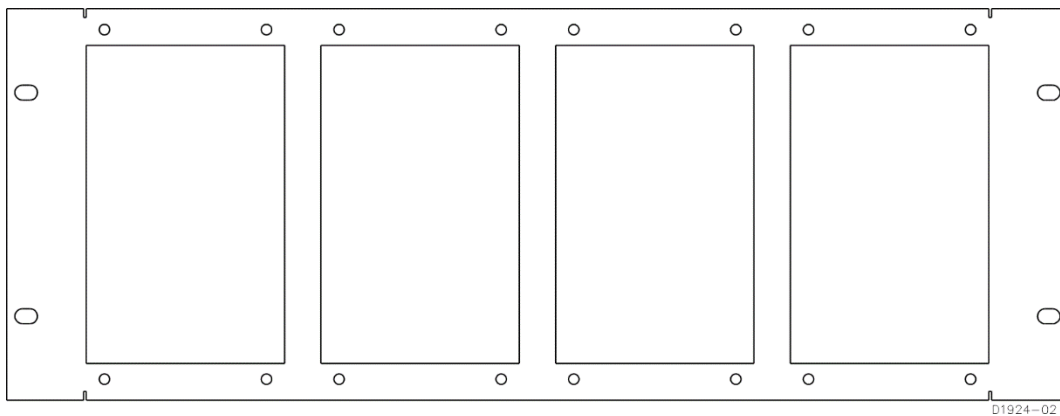
Figure 4-1. Rack Mounting Plate, Part Number 9252012001
