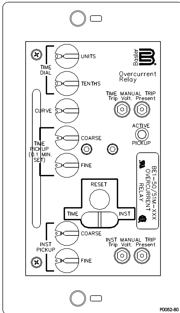
Figure 1-2. BE1-50/51M, C1 Vertical Mount Case
