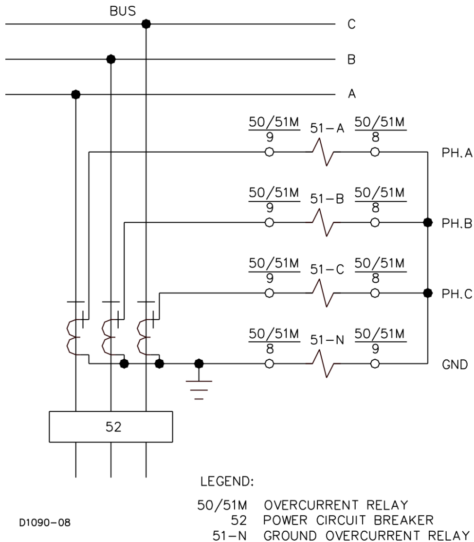
Figure 4-4. AC Input Connections
