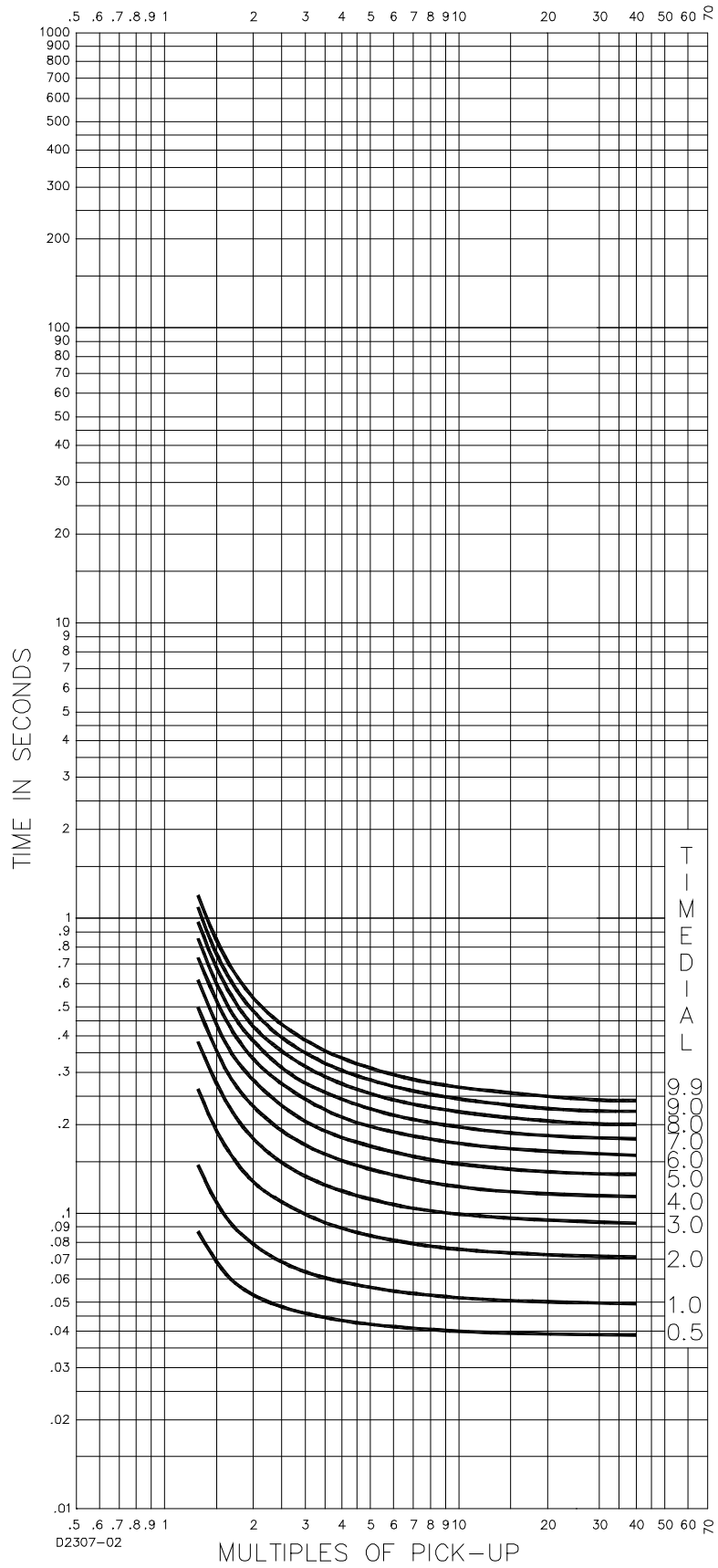
Figure 8-10. Time Characteristic Curve, S2-Short Inverse (SW3-3 ON, Similar to GE IAC 55)
