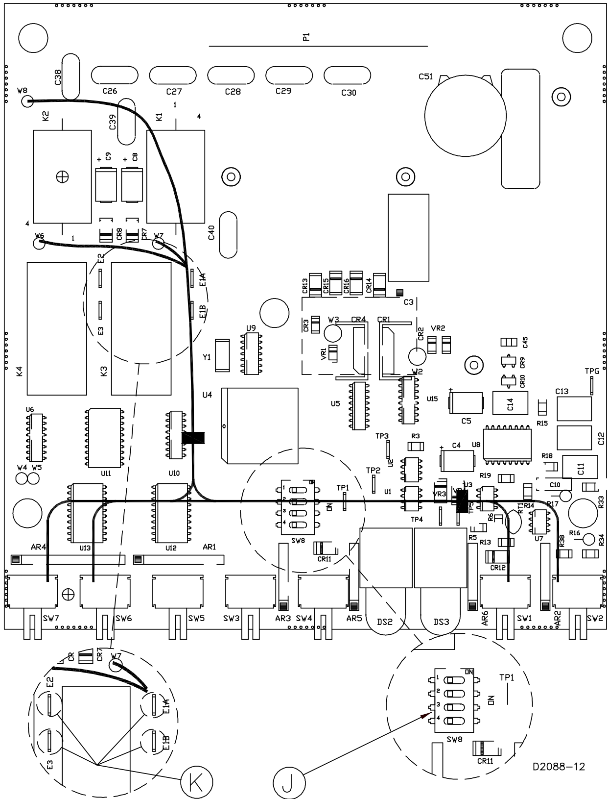
Figure 7-2. Location of Controls and Indicators for Unit Revision Q and Previous, 100 Series Relays
