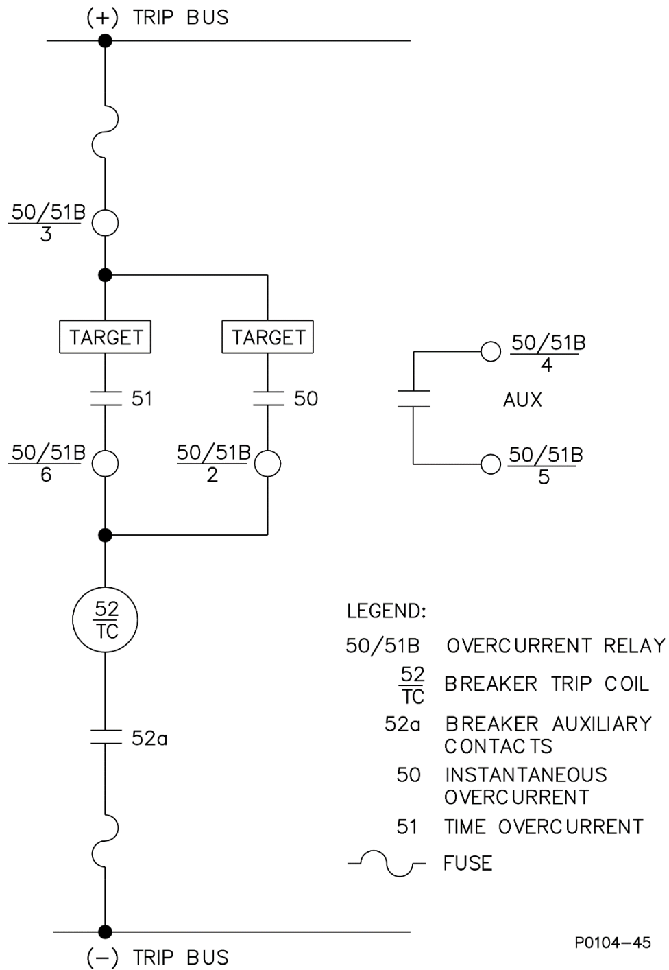
Figure 4-5. DC Control Connections
