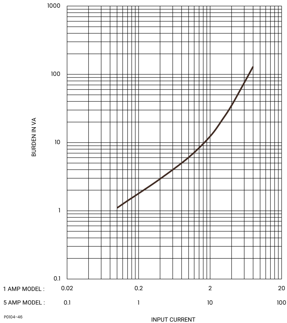
Figure 6-3. Burden Characteristics
