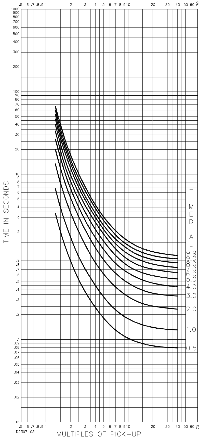
Figure 8-13. Time Characteristic Curve, V2-Very Inverse (SW3-3 ON, Similar to GE IAC 53)
