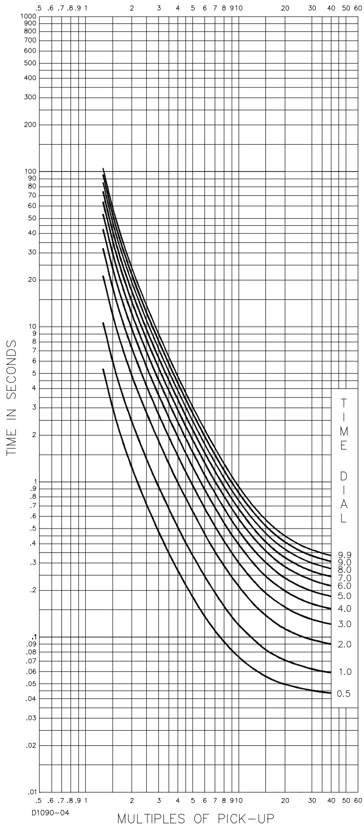
Figure 8-7. Time Characteristic Curve, E-Extremely Inverse (SW3-3 OFF, Similar to ABB CO-11)
