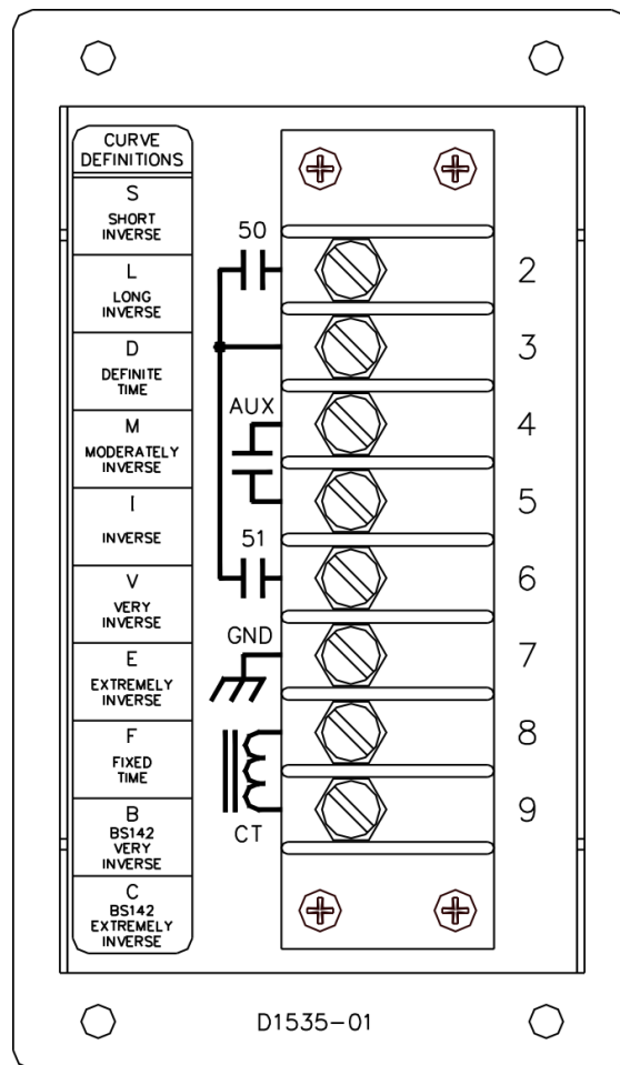
Figure 4-6. BE1-50/51M Terminal Connections, Rear View
