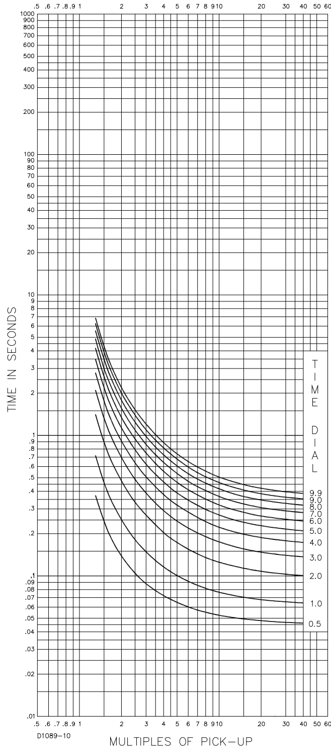
Figure 8-1. Time Characteristic Curve, S-Short Inverse (SW3-3 OFF, Similar to ABB CO-2)
