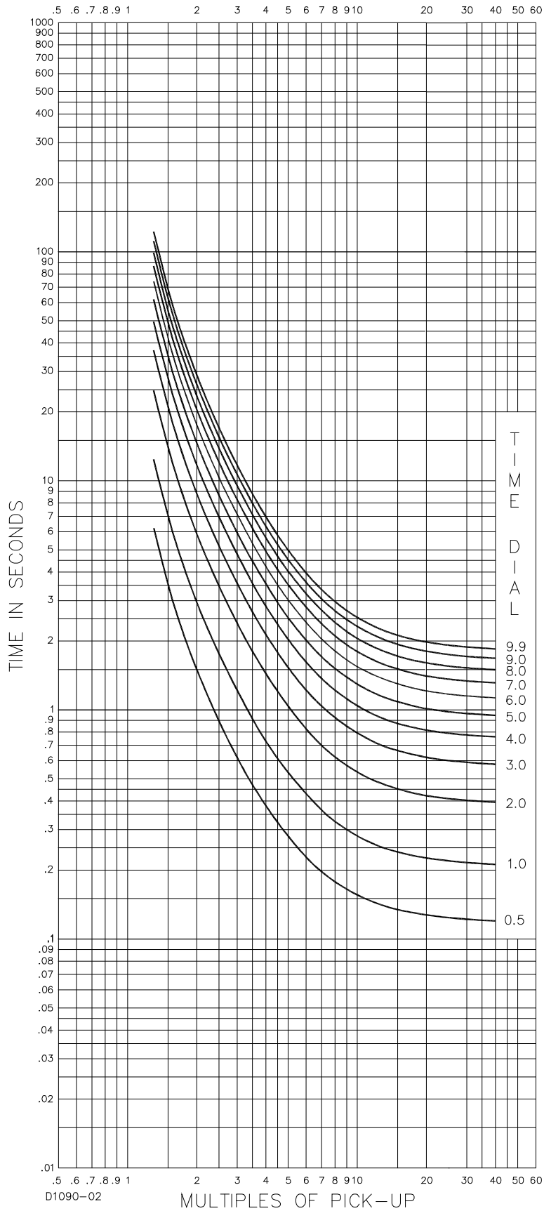
Figure 8-5. Time Characteristic Curve, I-Inverse (SW3-3 OFF, Similar to ABB CO-8)
