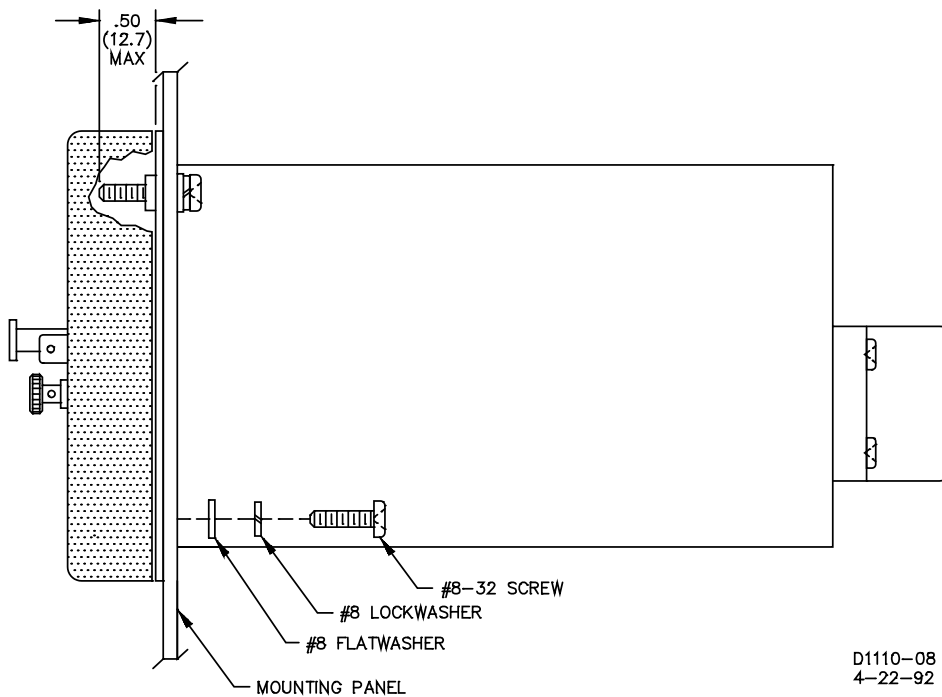
Figure 4-3. Panel Drilling Diagram, C1 Case
