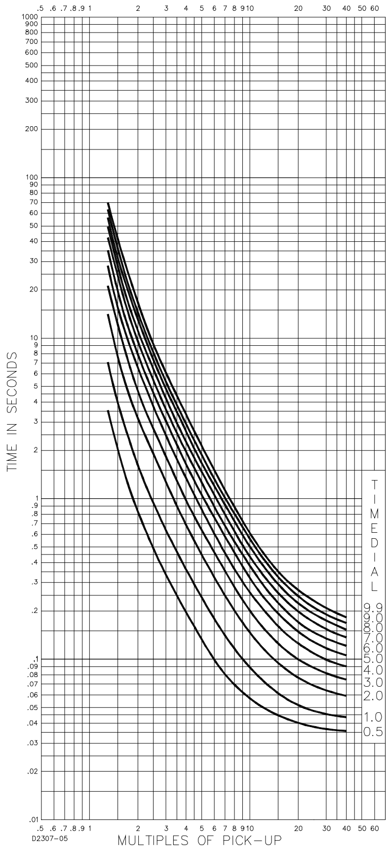
Figure 8-14. Time Characteristic Curve, E2-Extremely Inverse (SW3-3 ON, Similar to GE IAC 77)
