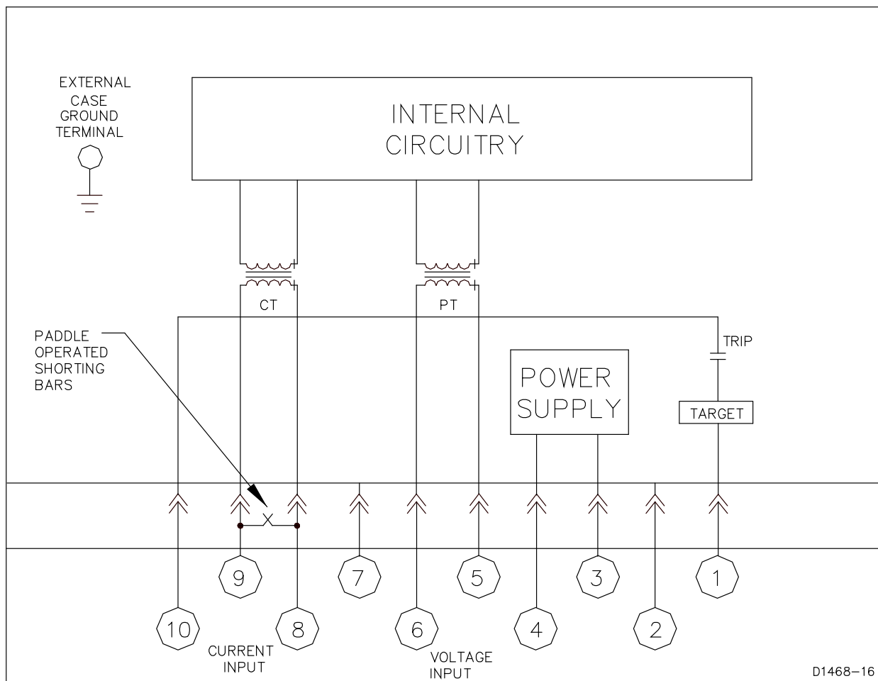
Figure 4-15. Interconnection with Current Operated Targets
