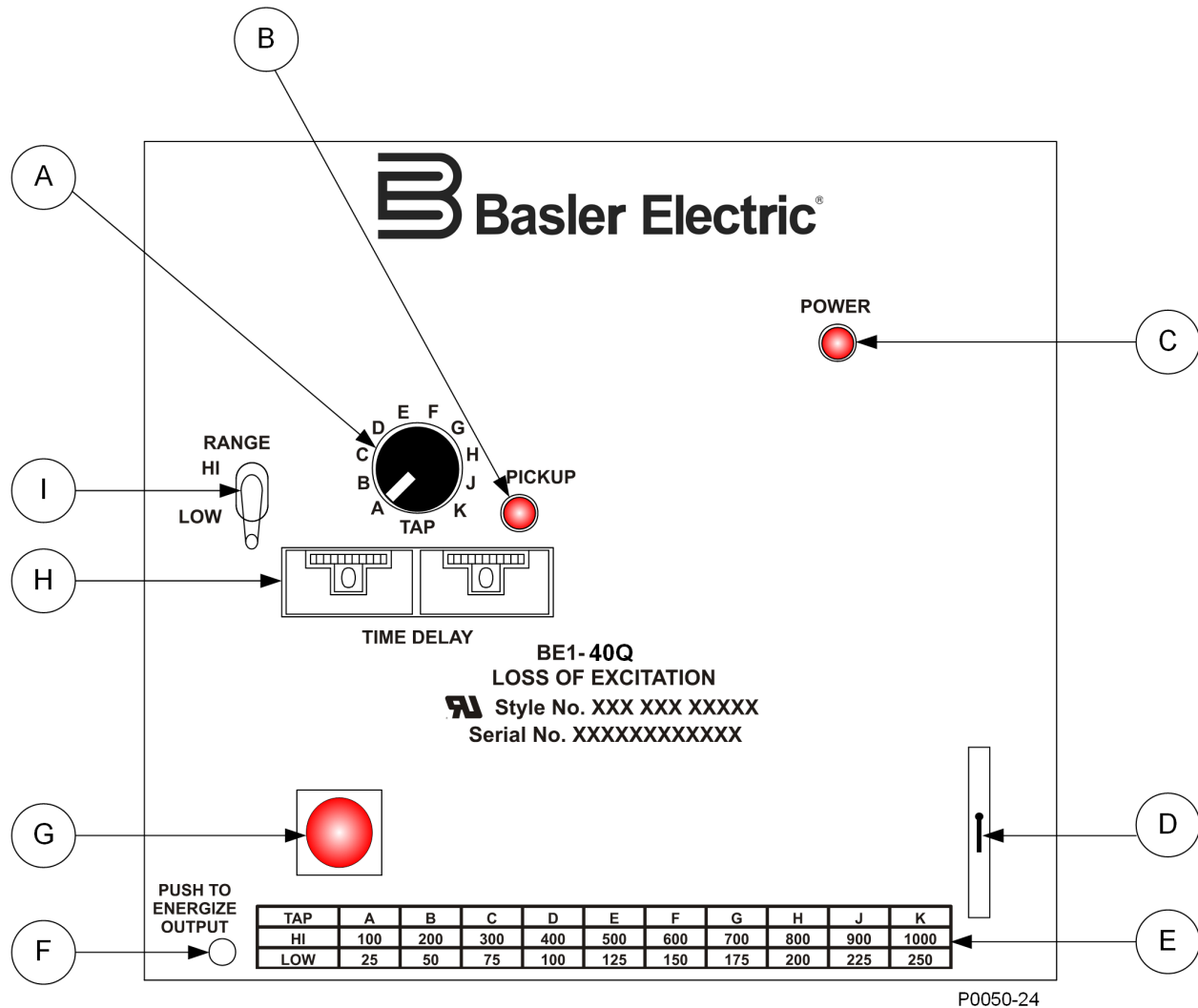
Figure 2-1. BE1-40Q Controls and Indicators
