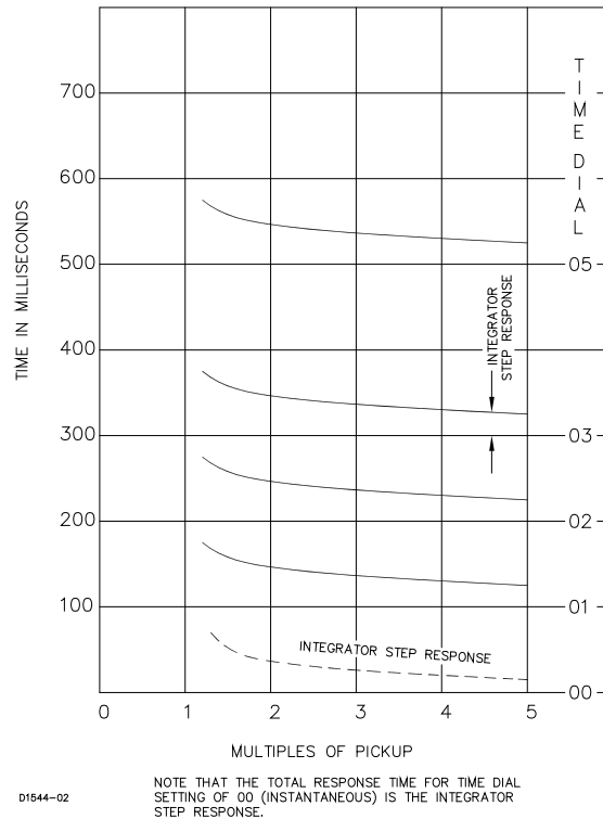
Figure 1-5. Typical Relay Response Time for Time Dial Settings
