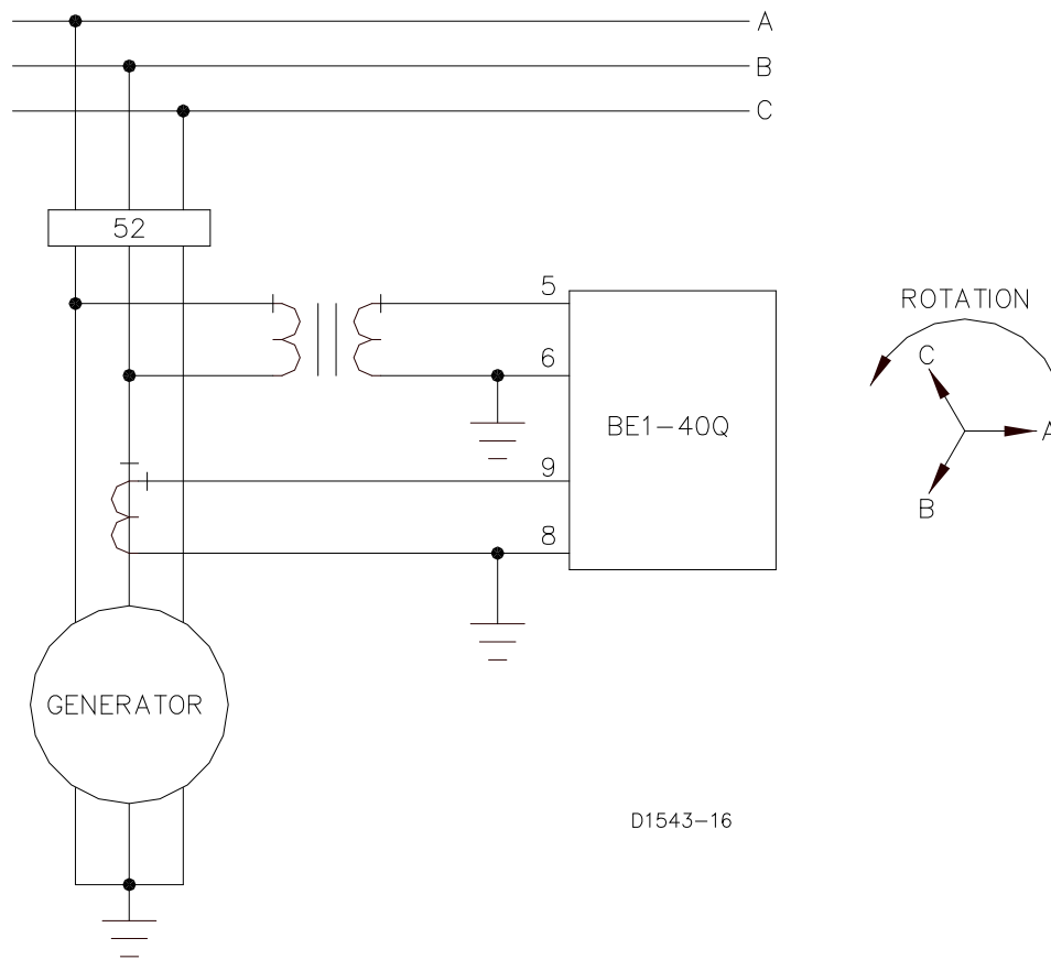
Figure 4-13. Sensing Input Connections
