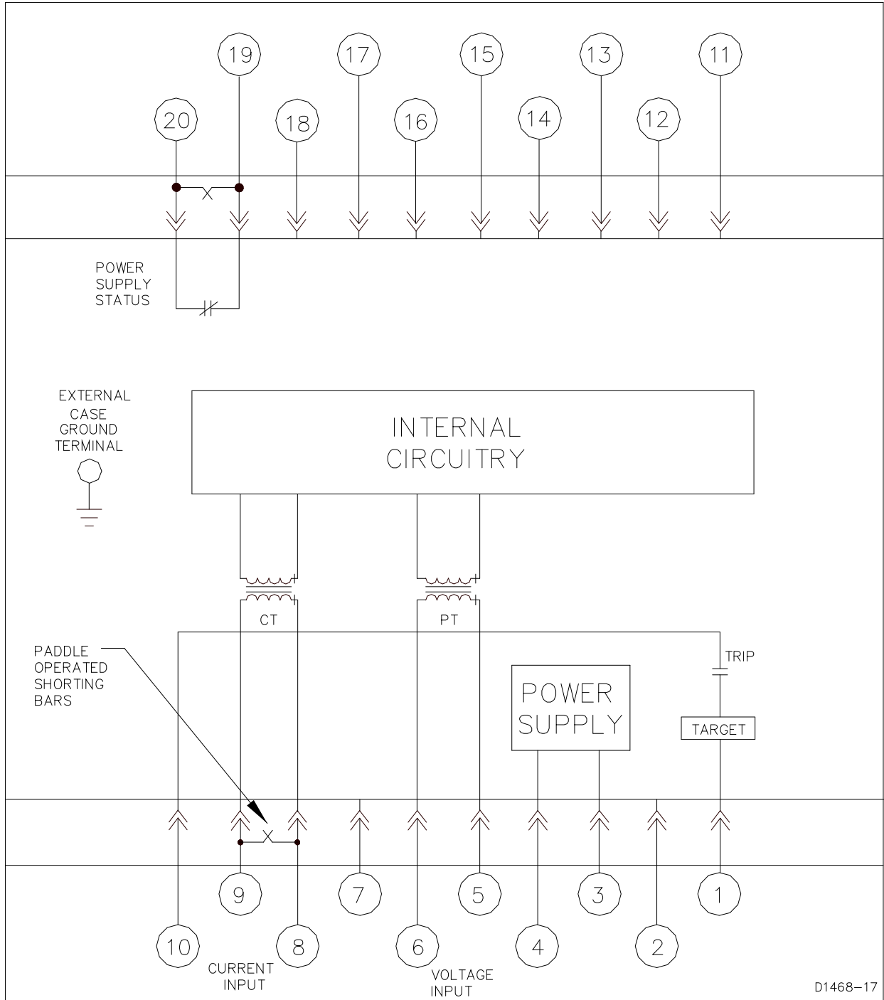
Figure 4-16. Interconnection with Current Operated Targets and Power Supply Status Output
