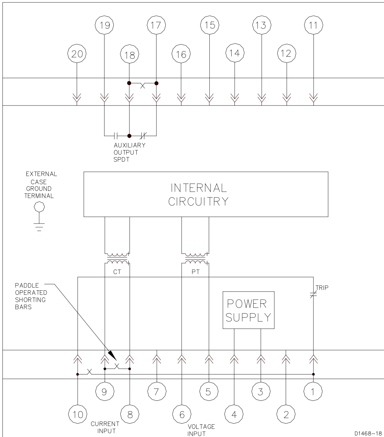
Figure 4-17. Interconnection with Internally Operated Target and Auxiliary Output Contacts (SPDT)
