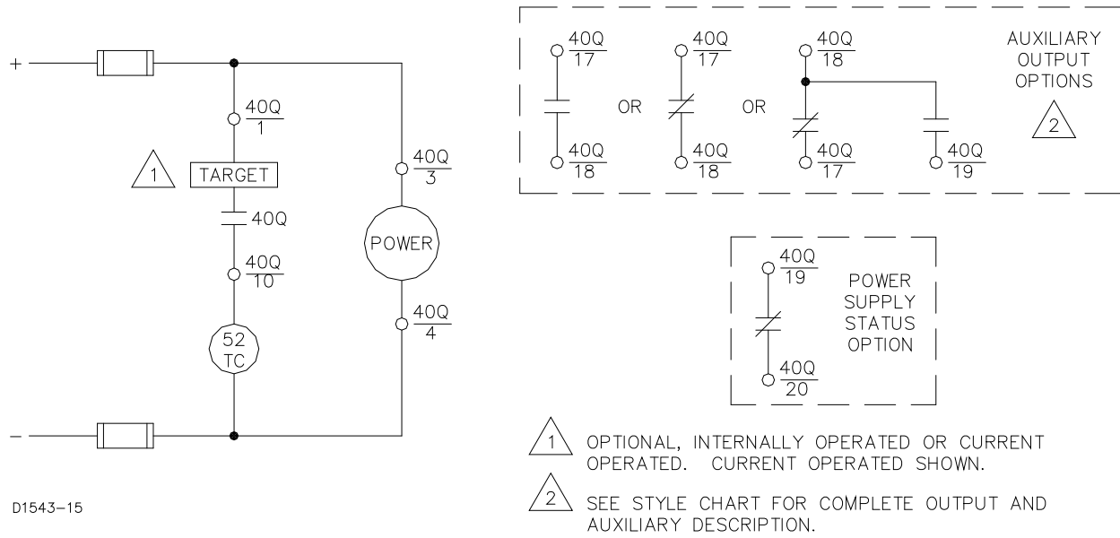
Figure 4-14. Output Connections
